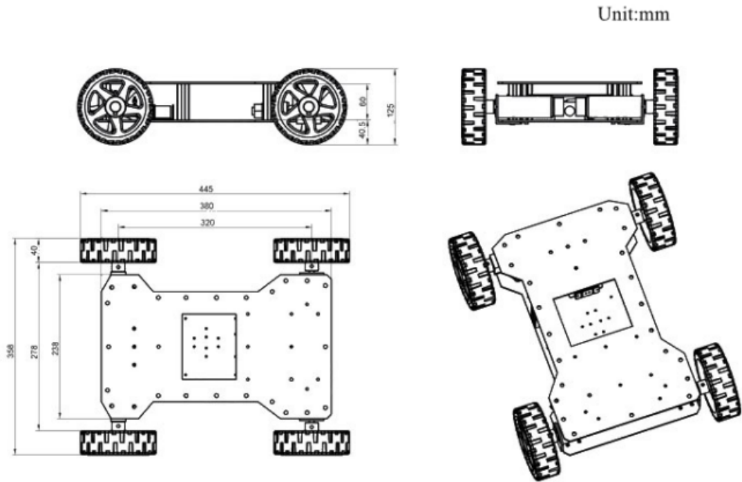
Rosbot Chassis Design Diagram:
