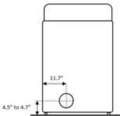
Venting location
