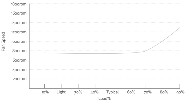
Power Supply Fan Curve
