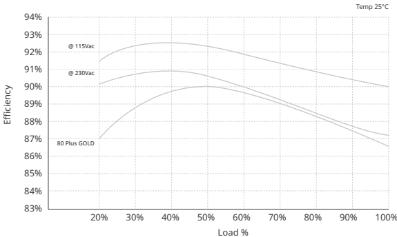
Power Supply Efficiency
