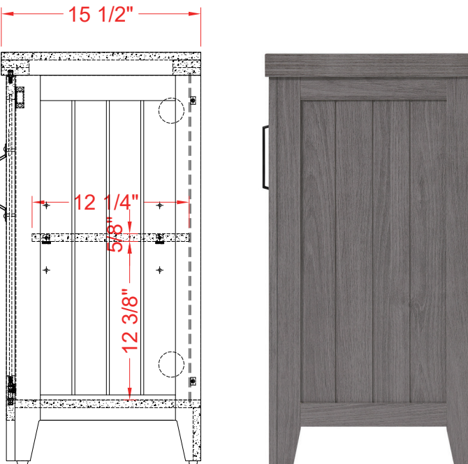
SIDE VIEW
