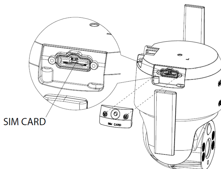
Figure 2-5 SIM card
