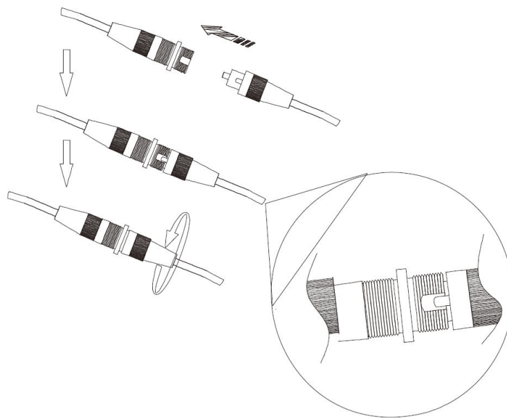
Figure 1-1 Connect cables
