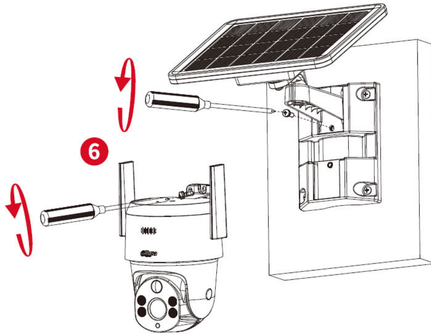
Figure 2-9 Wall mount (2)
