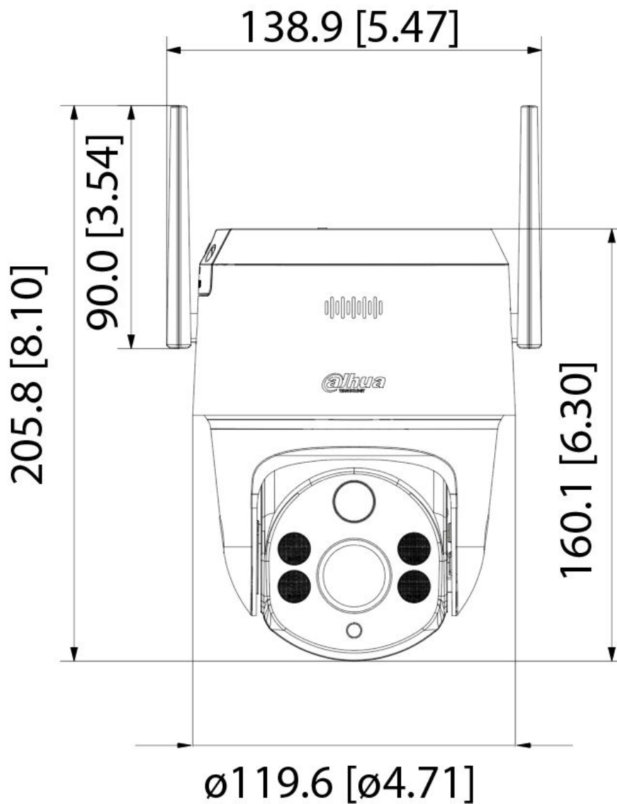
Figure 2-2 Dimensions (mm [inch])
