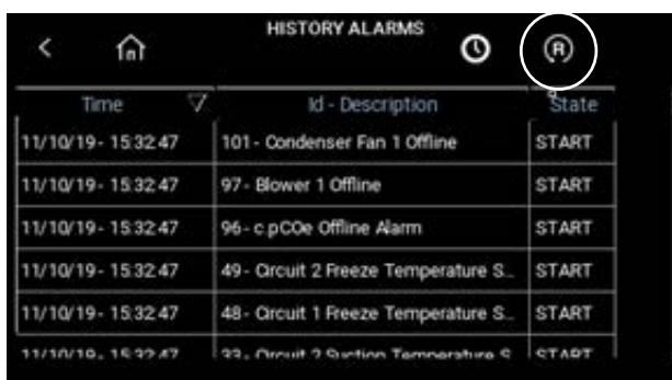
FIGURE 24 Resetting Alarm History Log
