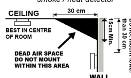
Figure 3i Positioning the smoke / heat detector
