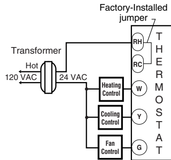
HEAT/COOL 4-WIRE SINGLE TRANSFORMER
