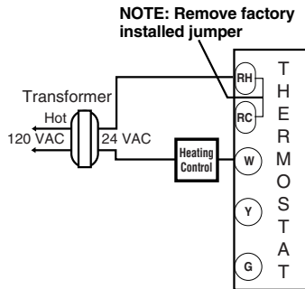
HEAT ONLY 2-WIRE SINGLE TRANSFORMER
