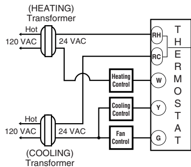
HEAT/COOL 5-WIRE TWO TRANSFORMER
