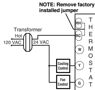
COOL ONLY 3-WIRE SINGLE TRANSFORMER
