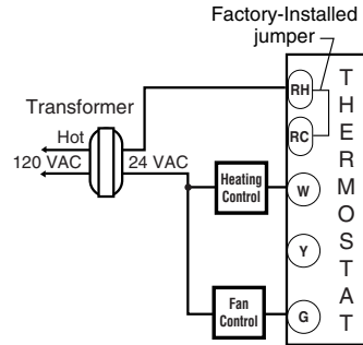
HEAT ONLY 3-WIRE SINGLE TRANSFORMER
