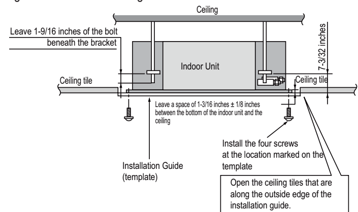
Figure 173: Installation Diagram.
