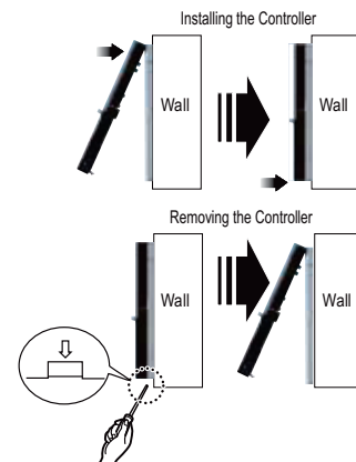
Figure 58: Installing/Removing the Controller.
