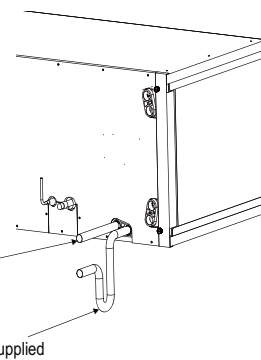
Figure 243: Insulating the Refrigerant Piping and Refrigerant Piping Connections.
