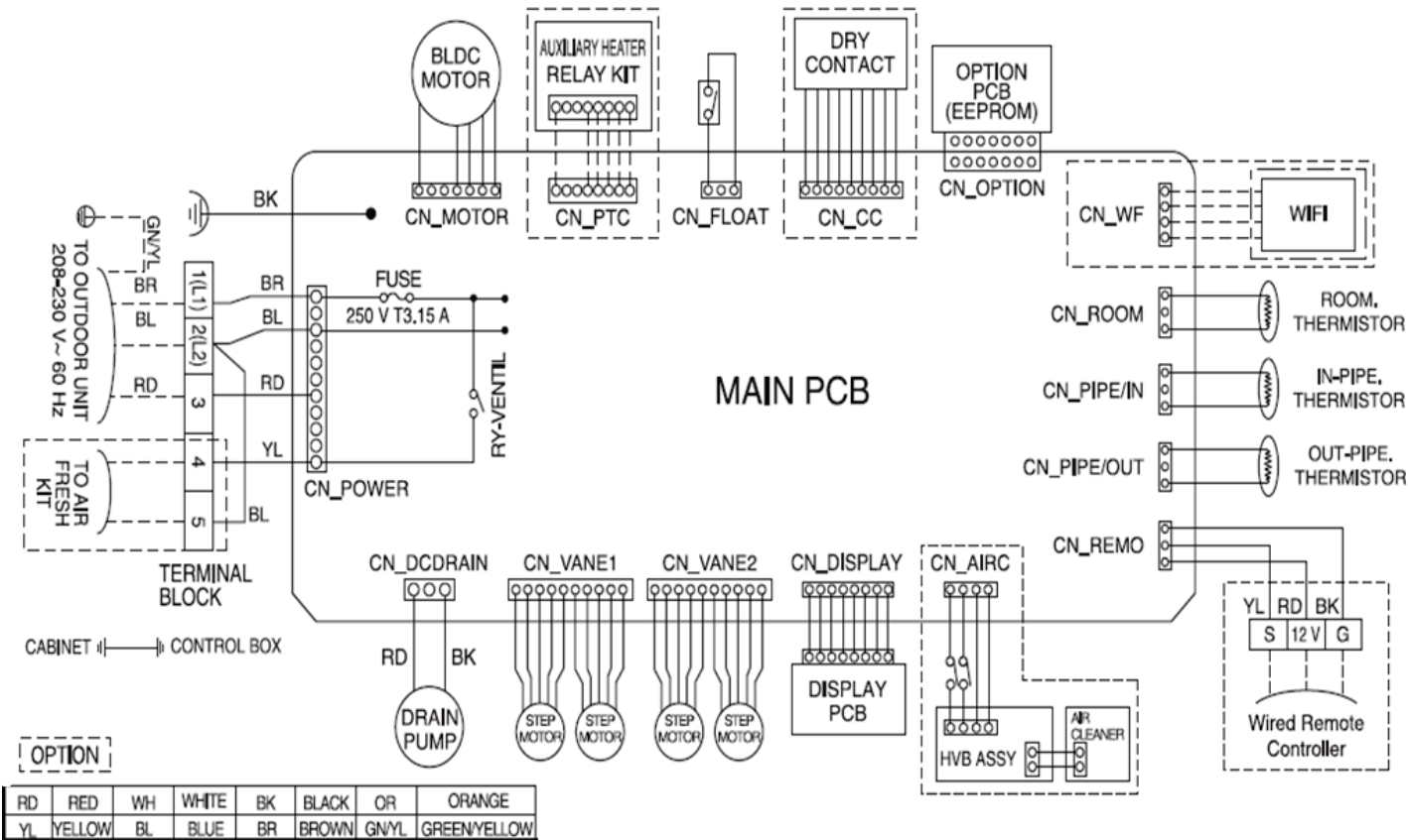
Figure 167: Multi F Four-Way Ceiling-Cassette Indoor Unit Wiring Diagram.
