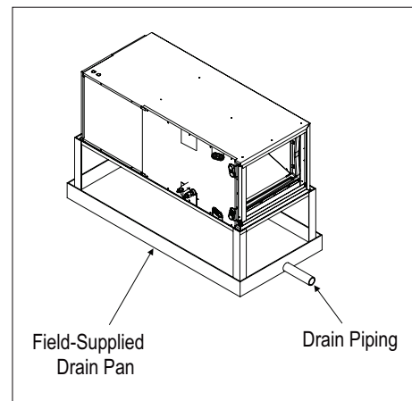
Figure 237: Typical Horizontal Left/Right Installation Drain System.
