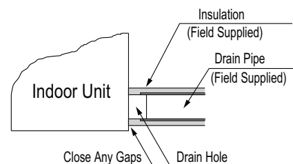
Figure 110: Drain Connection.
