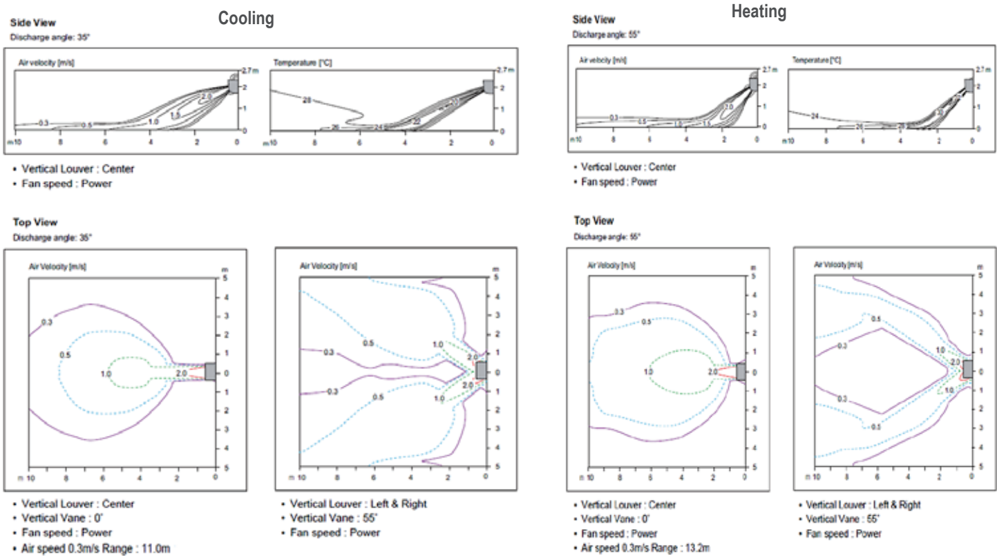
Figure 6: LAN090HSV5 and LAN120HSV5 Air Velocity and Temperature Distribution Charts.
