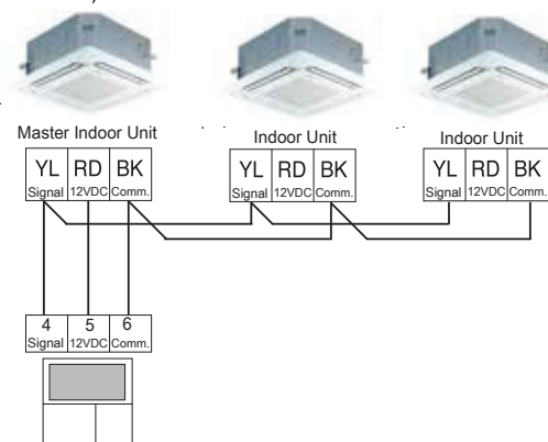
Figure 279: Example of Indoor Unit Group to Zone Controller Connections (Sig-12V-GND [Comm.] Terminal).
