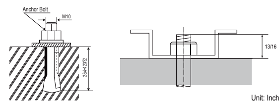
Figure 255: Close up of Bolt Attachment.
