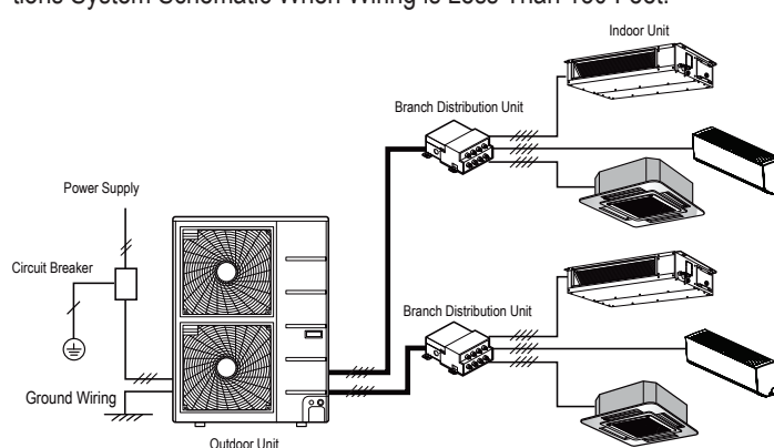
Figure 263: Typical Multi F MAX System General Power / Communications System Schematic When Wiring is Less Than 130 Feet.
