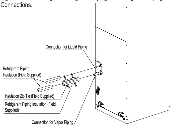
Figure 243: Insulating the Refrigerant Piping and Refrigerant Piping Connections.
