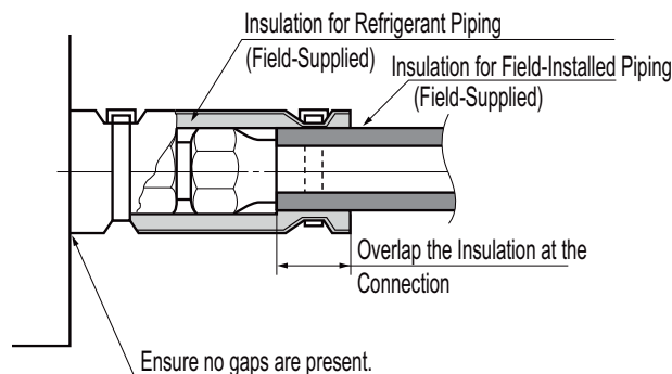
Figure 177: Insulating the Piping.
