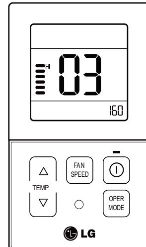
Figure 155: Controller External Static Pressure Setting Display.
