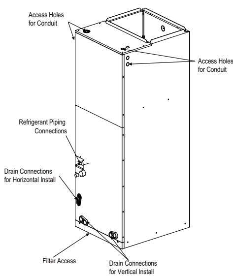
Figure 197: General and Duct Connection Dimensions.
