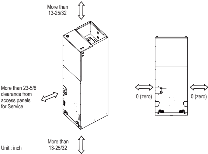
Figure 228:Clearance Requirements.
