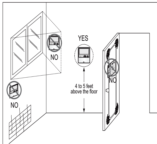
Figure 149: Proper Location for the Wired Controller.
