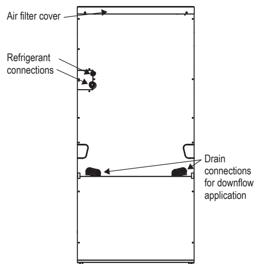
Figure 232: Chassis after Downflow Field Conversion.
