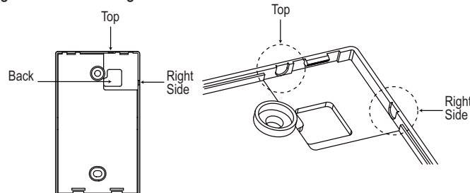
Figure 152: Installing / Removing the Controller.
