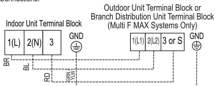
Figure 116: Indoor Unit to Outdoor Unit / Branch Distribution Unit (Multi F MAX systems only) Power Wiring / Communications Cable Connections.
