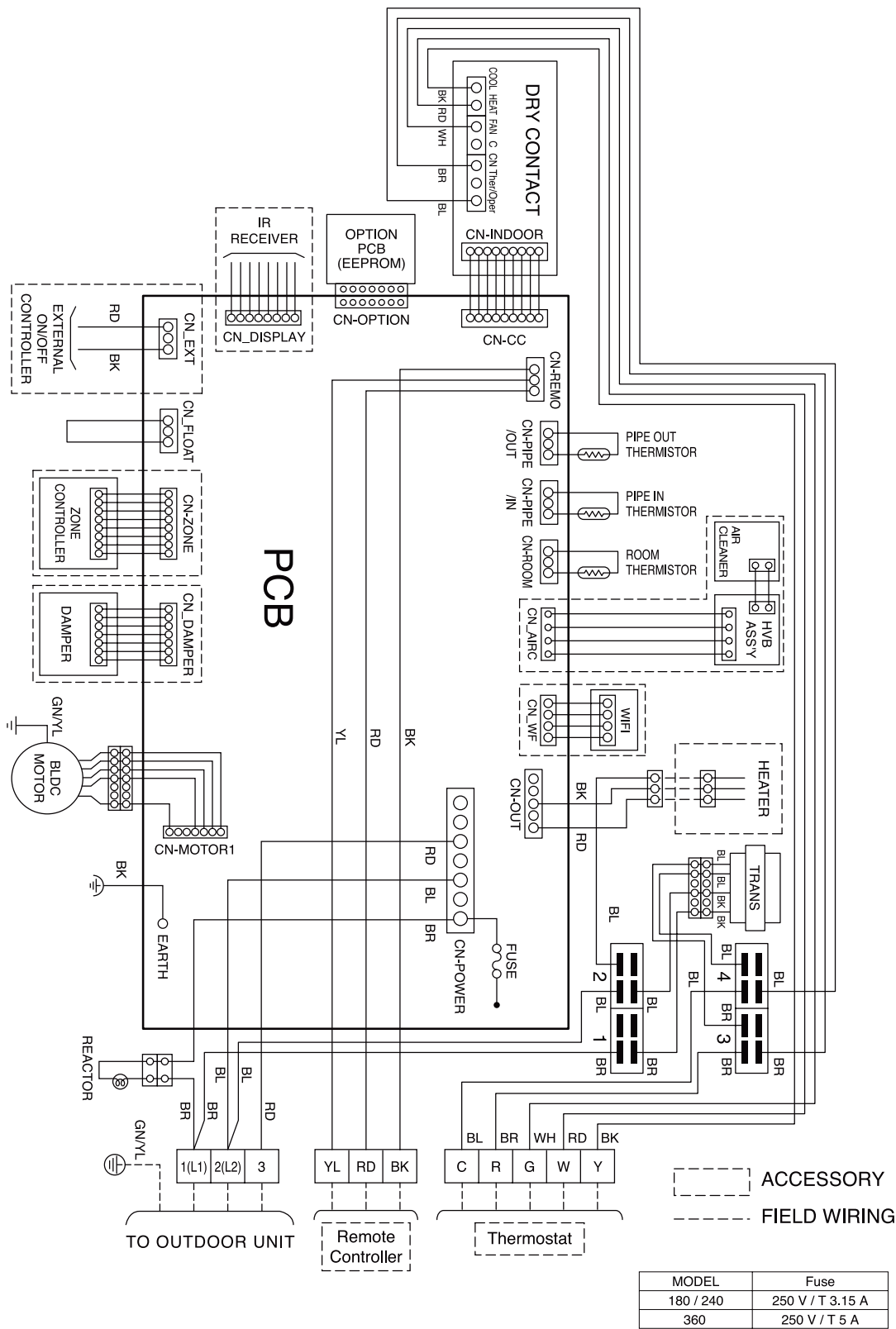
Figure 227: Four-way Vertical-Horizontal Air-Handling Indoor Unit Wiring Diagram.
