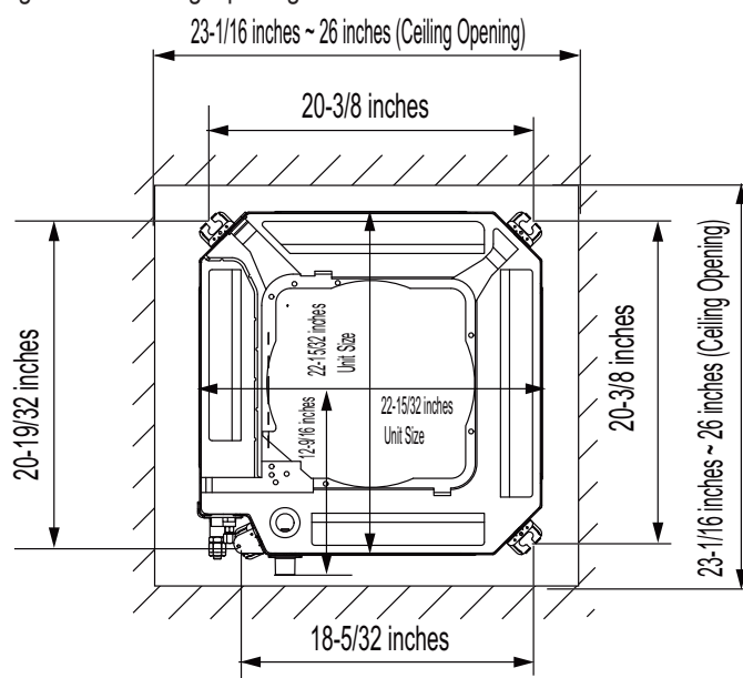
Figure 171: Ceiling Opening Dimensions and Bolt Locations.
