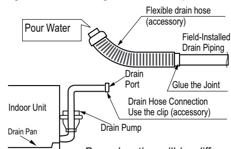
Figure 113: Checking the Drain Pump.
