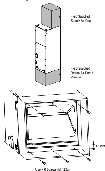
Figure 231: Vertical Installation / Attaching the Bottom Duct.
