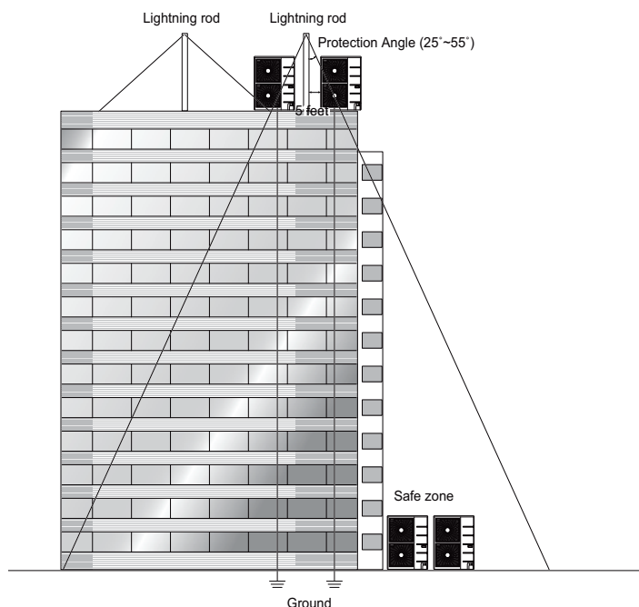
Figure 256: Lightening Protection Diagram.
