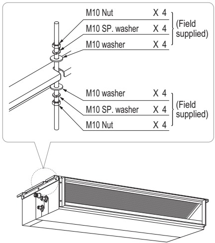
Figure 109: Hanging the Indoor Unit.
