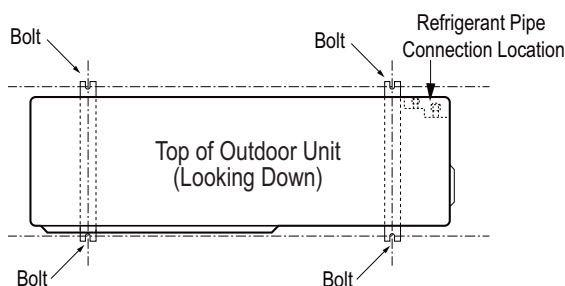
Figure 255: Close up of Bolt Attachment.
