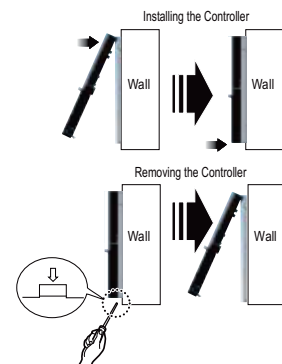
Figure 217: Installing / Removing the Controller.
