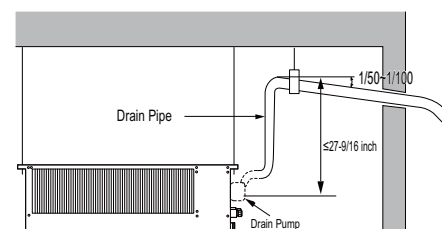
Figure 111: Indoor Unit Using Drain Pump.
