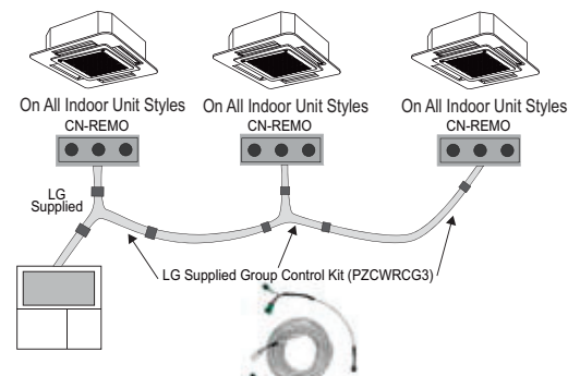
Figure 280: Example of Indoor Unit Group to Zone Controller Connections (CN-REMO).
