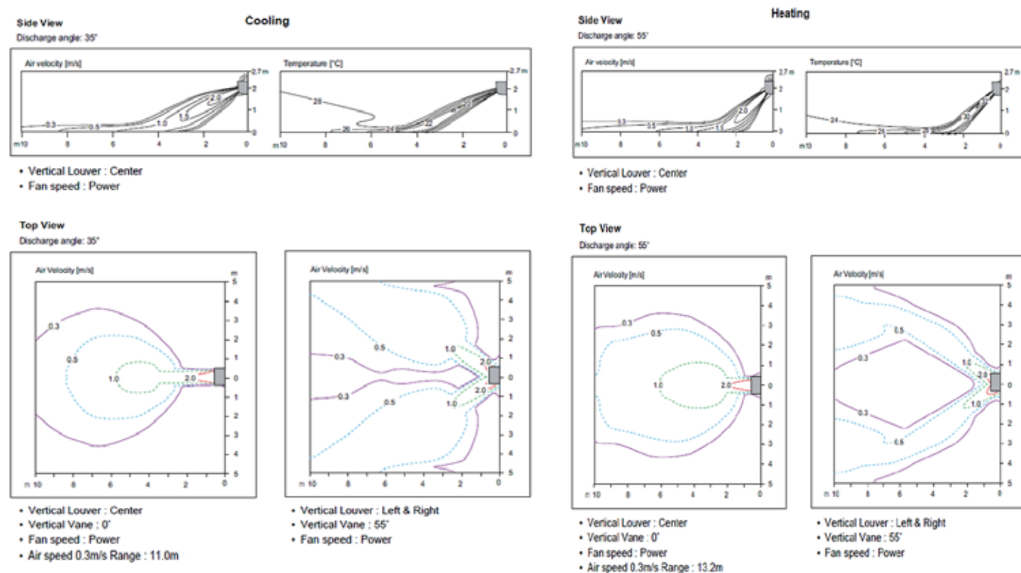
Figure 66: LMN079HVT, LSN090HSV5, LSN120HSV5, LMN159HVT Air Velocity and Temperature Distribution Charts.
