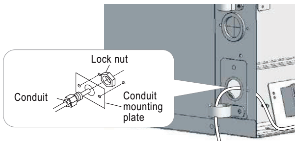
Figure 117: Exterior View of Conduit Installation.
