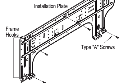
Figure 73: Installation Plate— Side View.
