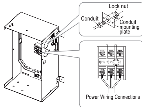
Figure 146: Exterior View of Conduit Installation.
