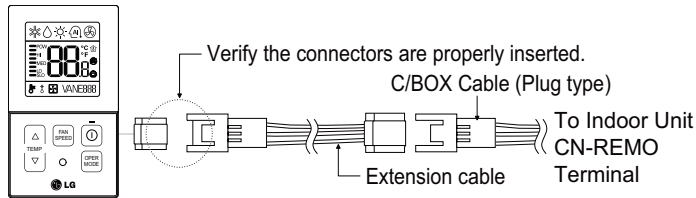
Figure 118: PZCWRC1 LG Wired Remote Extension Cable.
