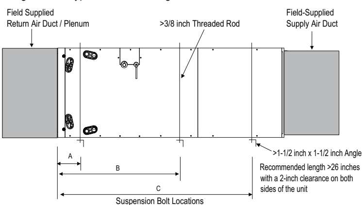
Figure 234: Typical Horizontal Right Installation.
