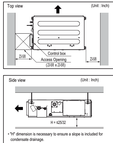
Figure 103: General Installation Guidelines.
