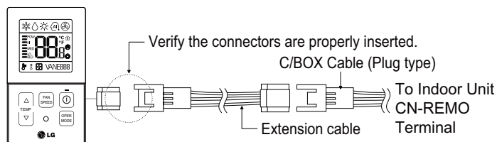
Figure 148: Wired Controller Connections on the Indoor Unit Terminal Block.
