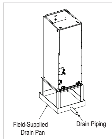
Figure 202: Vertical Installation Drain System.
