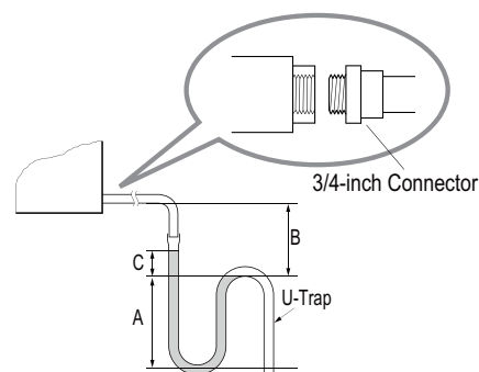
Figure 241: Horizontal Primary and Secondary Drain Layout.
