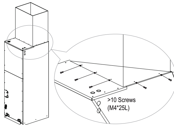
Figure 235: Securing the Ducts to the Unit.
