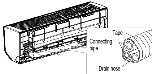
Figure 81: Piping Installed to the Left.
