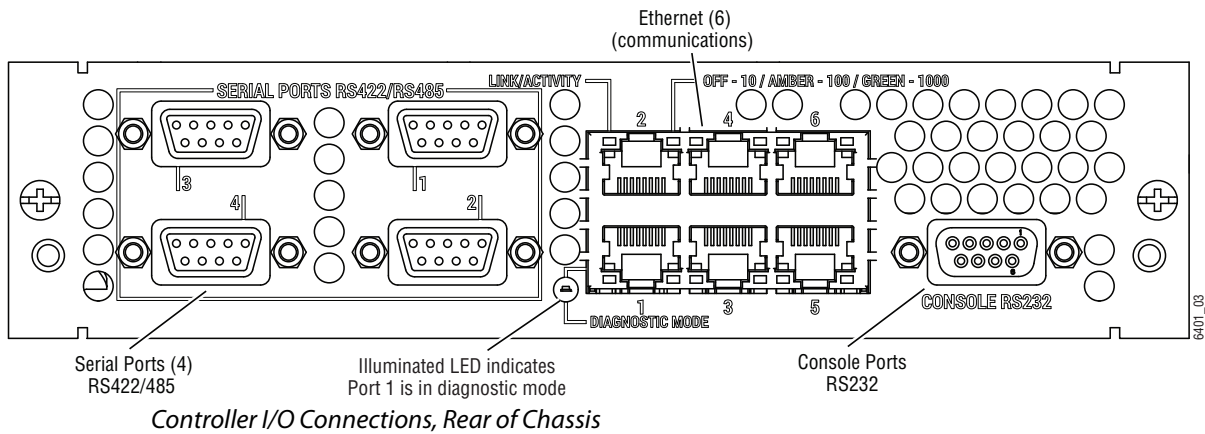
K-Frame V-series 3-RU, Rear View
