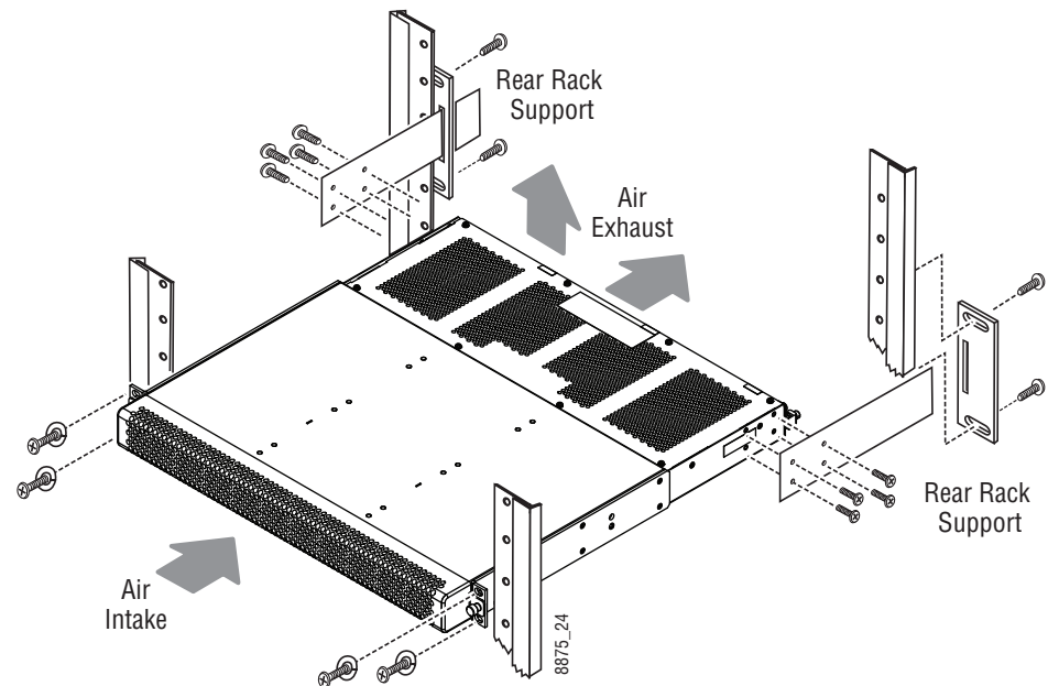
Isolated K-Frame 13-RU Power Supply Rack Installation
