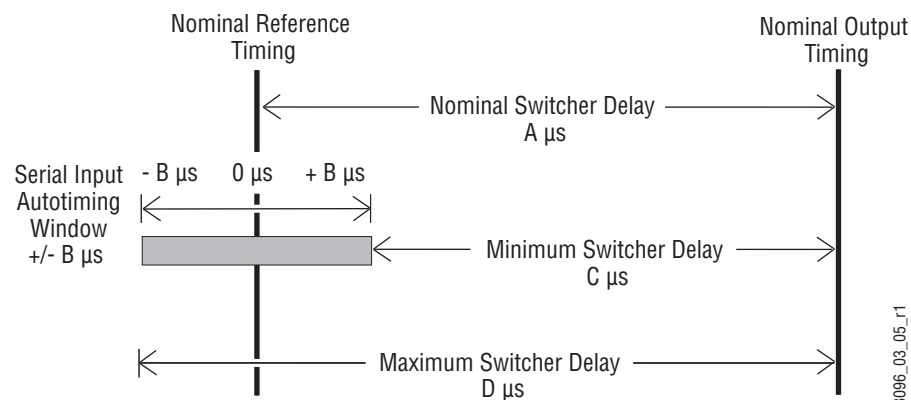
Switcher Timing Diagram
