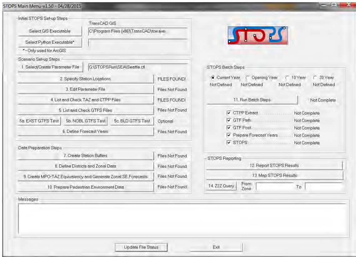
Figure 24. STOPS Main Menu After All TAZ and CTPP Files Are Loaded
