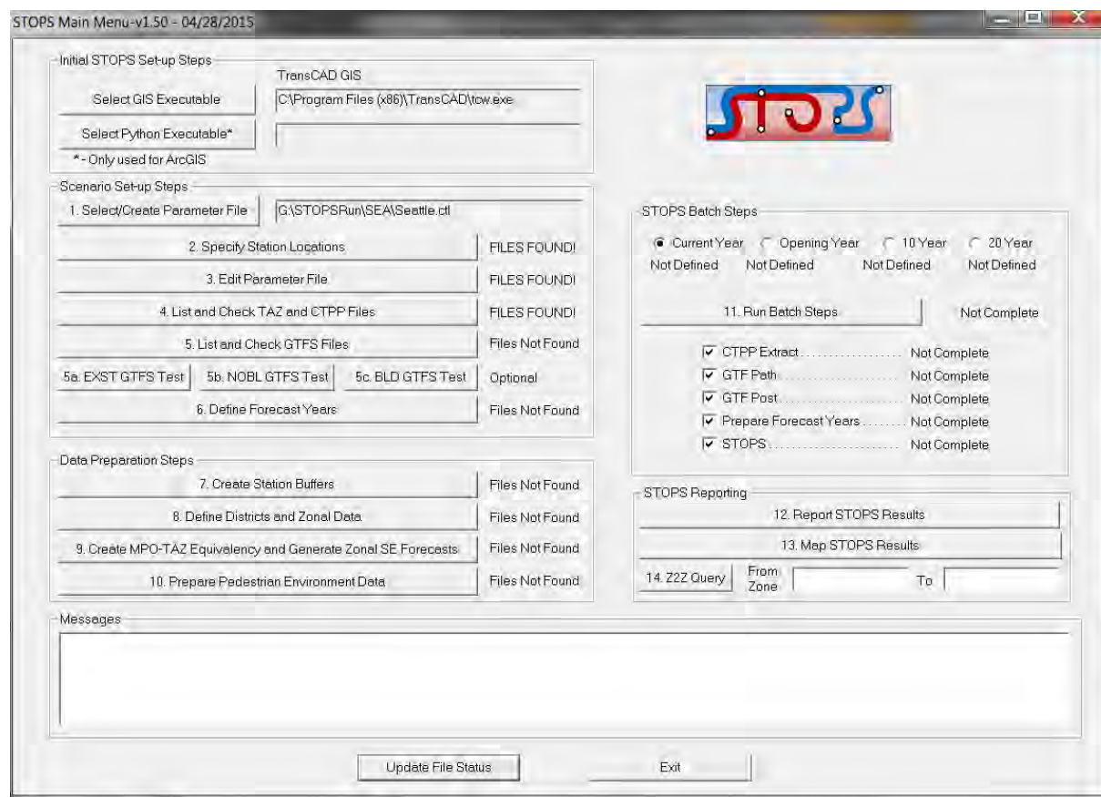
Figure 58. STOPS Main Menu After All GTFS Files are Found
