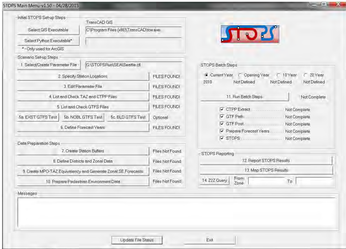
Figure 62. STOPS Main Menu At Beginning of Data Preparation
