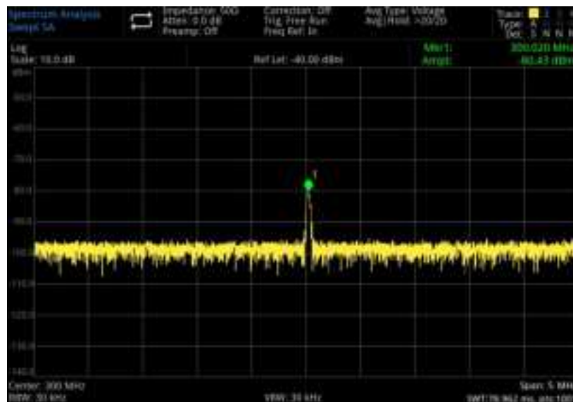
Figure 3-14 Trace Averaging
