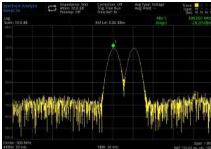
Figure 3-6 Distinguished Two Equal-Amplitude Signal (1)
