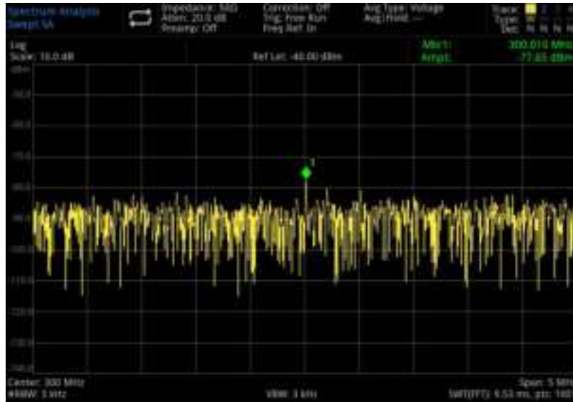
Figure 3-13 Reduce Resolution Bandwidth
