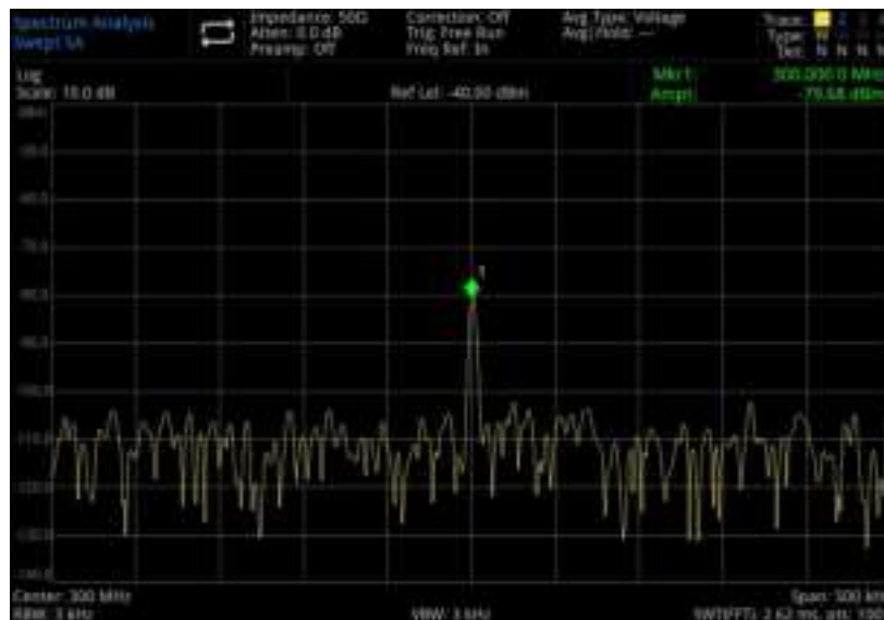
Figure 3-12 Measuring Small Signal with 0dB Attenuation
