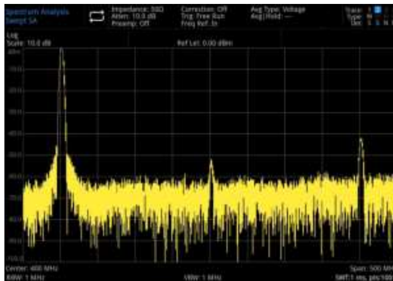
Figure 3-16 Harmonic Distortion
