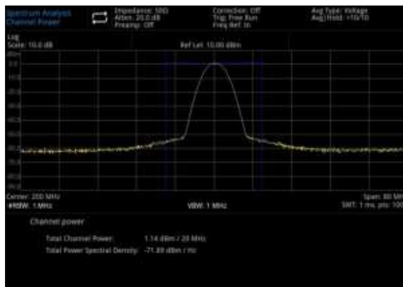
Figure 5-1 Channel Power
