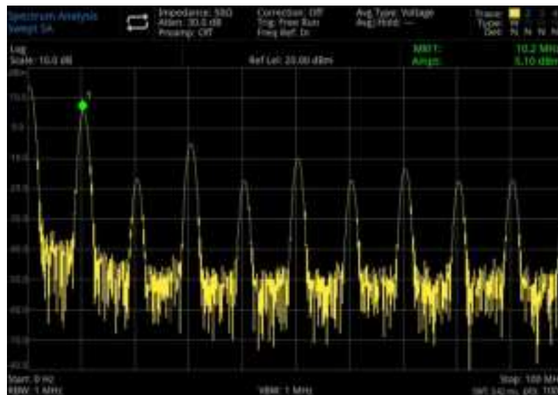
Figure 3-1 Read Frequency and Amplitude
