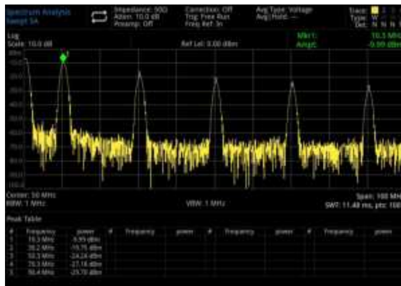
Figure 4-3 Peak List
