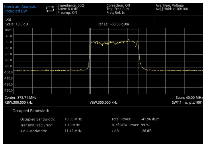
Figure 5-3 Occupied Bandwidth
