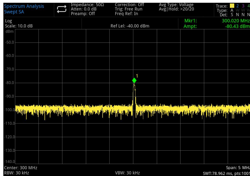
Figure 3-14 Trace Averaging
