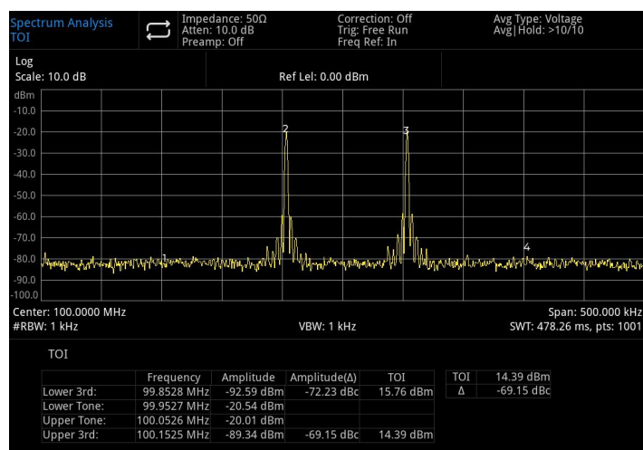
Figure 5-4 TOI
