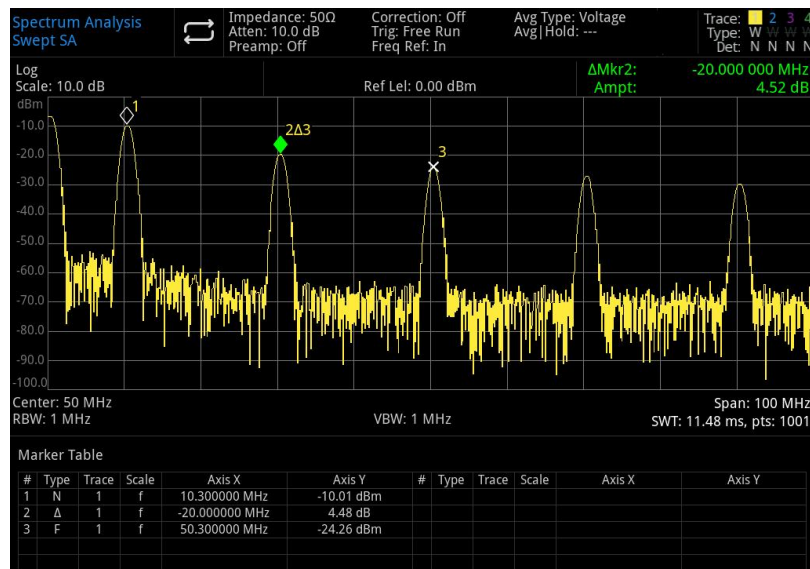
Figure 4-2 Marker List
