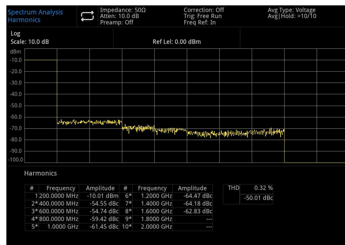
Figure 5-8 Harmonic Measurement
