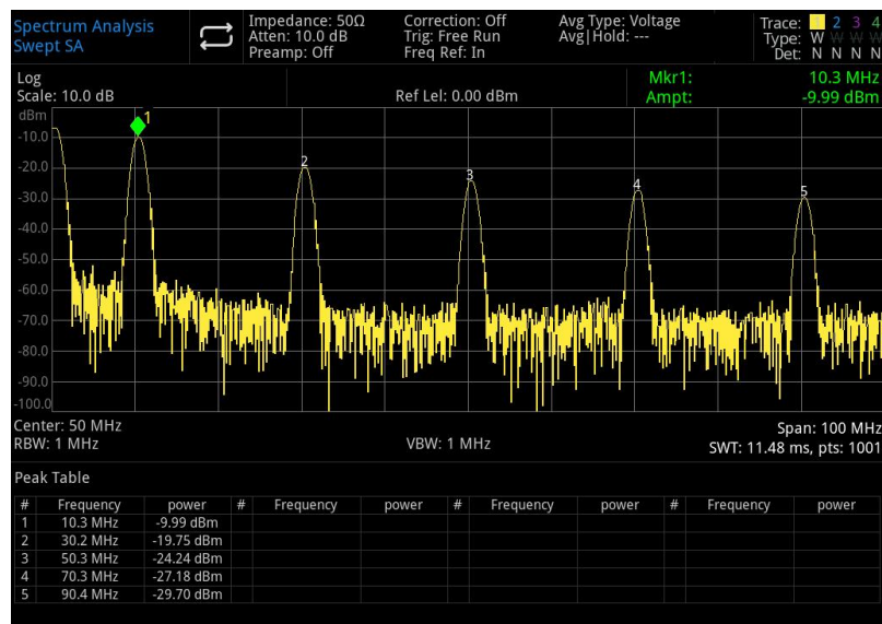
Figure 4-3 Peak List
