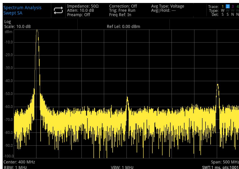
Figure 3-16 Harmonic Distortion
