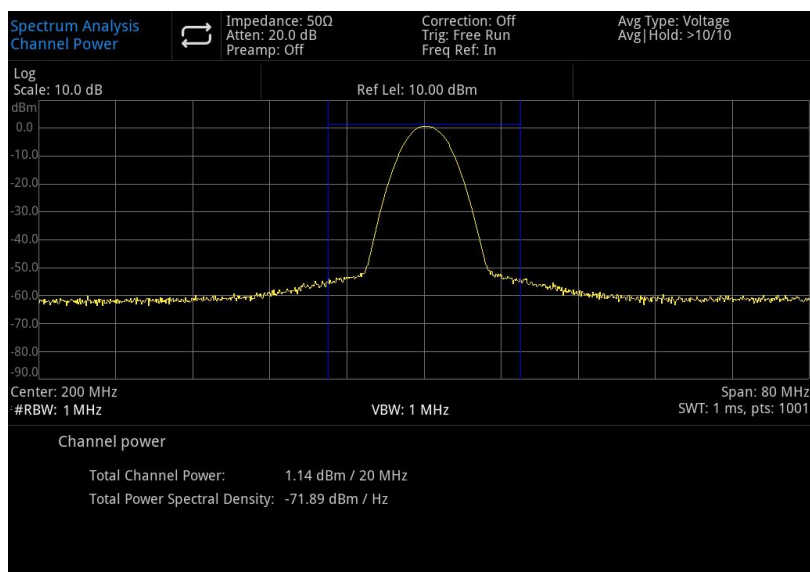
Figure 5-1 Channel Power
