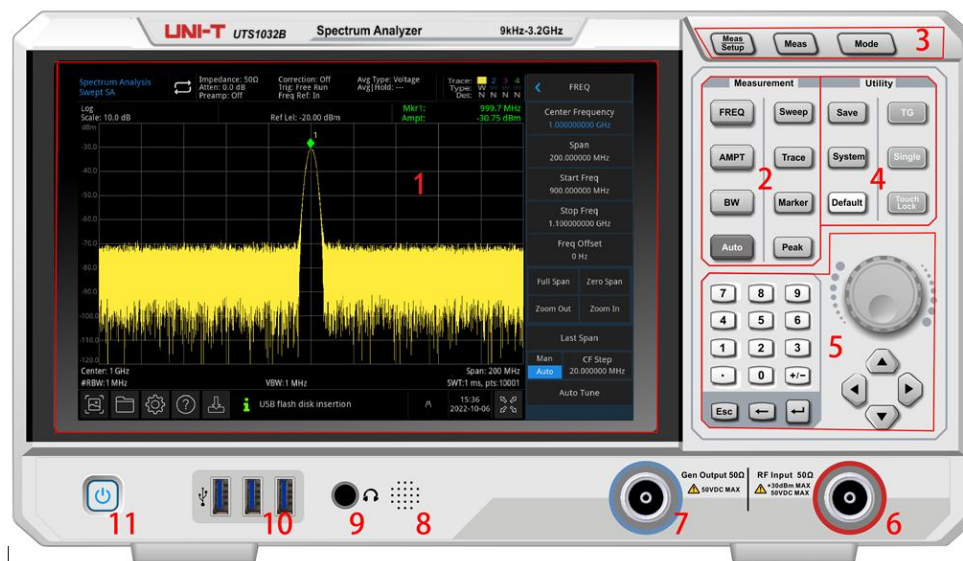
Figure 1-1 Front Panel
