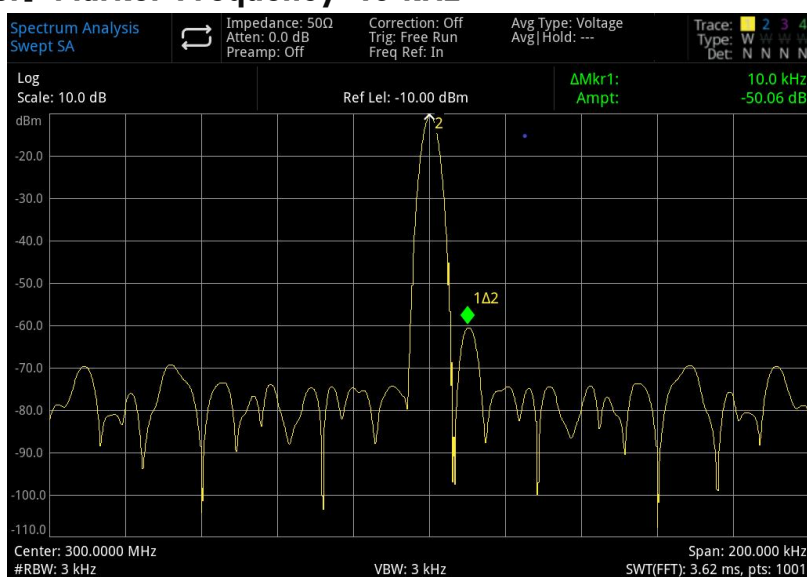
Figure 3-9: Distinguish Small Signal from Big Signal
