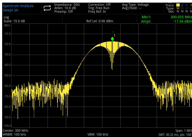
Figure 3-5 Undistinguished Two Equal-Amplitude Signals
