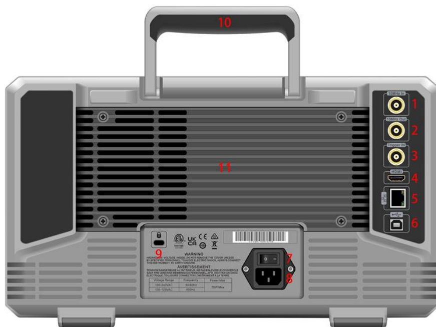
Figure 1-3 Rear Panel
