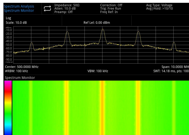
Figure 5-6 Spectrum Monitoring
