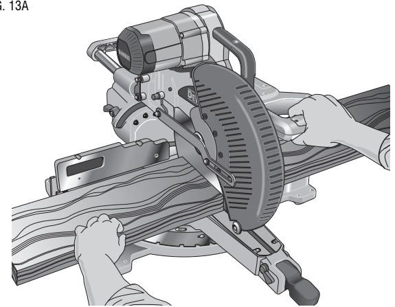
PROPER CUT
