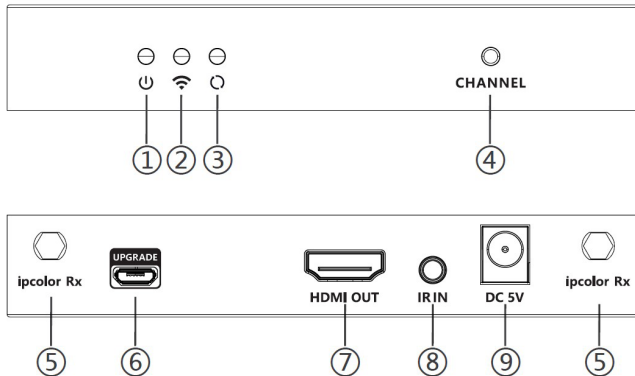
Figure 2: Receiver (RX)
