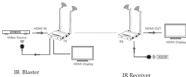
Figure 3: Connection Diagram
