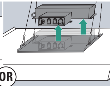
3. Set the driver and dimmer on the LED panel (or remove them off)
