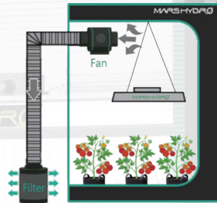
Works as Exhaust Filter System with Carbon Filter inside and Fan Outside
