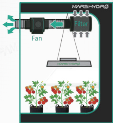
Works as Exhaust Filter System with Carbon Filter and Fan inside
