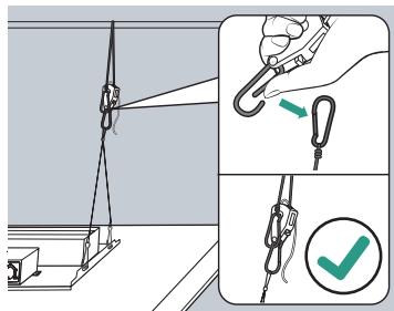
6. Hang the light with YOYO (Correct way to use YOYO)
