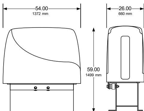
95xx-xxx with Standard Polyurethane housing
