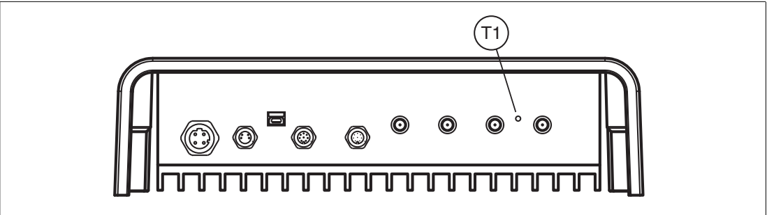
Figure 3.6 The configuration can be reset using the T1 button. The T1 button is located centrally between the ANT3 and ANT4 antenna connections. Use a paper clip, for example, to press the button.
