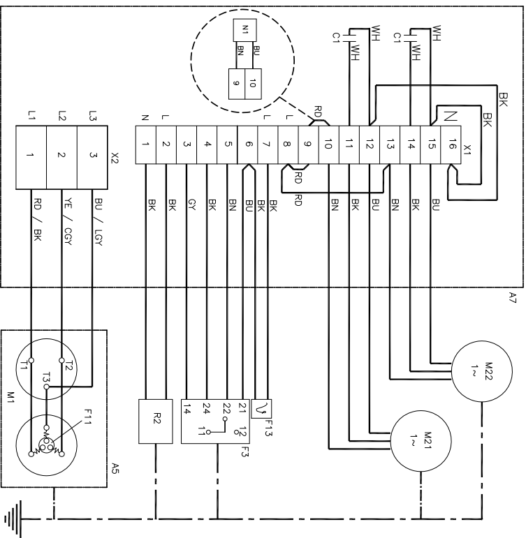
Typical Control Circuit
