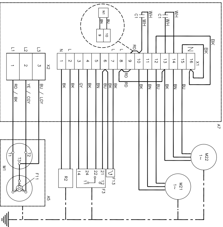
Typical Control Circuit
