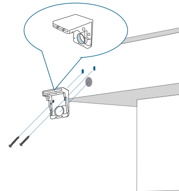
Wall Mounting
