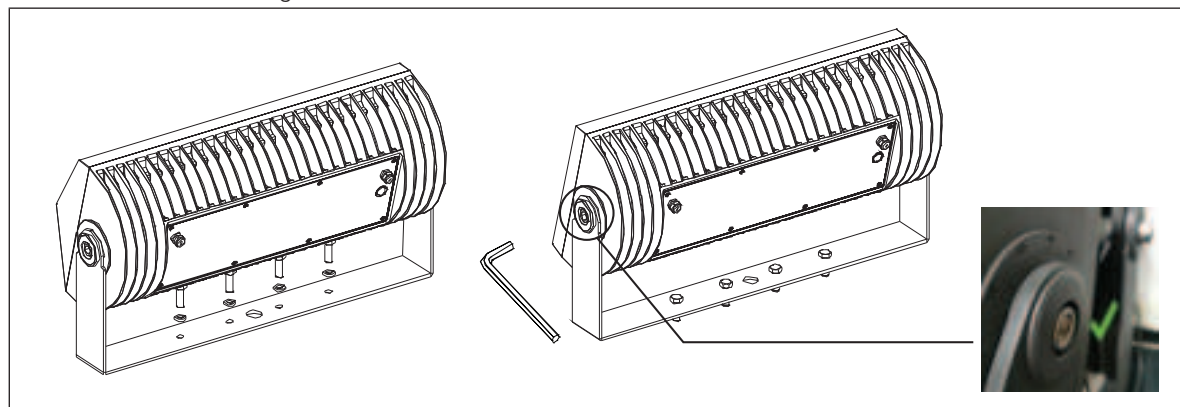
FIG.10: Bracket Mounting
