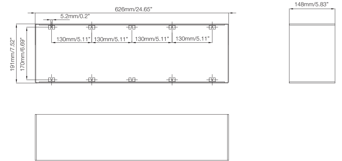
FIG.4: ProPoint Vista 100W Accessories-Full/Half Glare Shield
