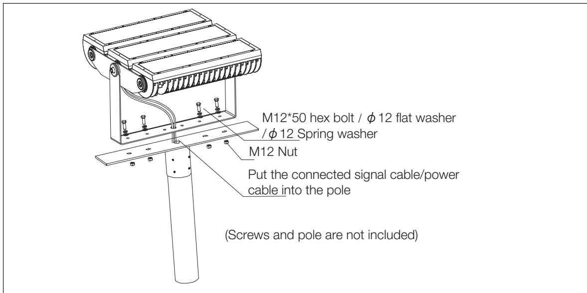
FIG.16: Pole Mounting Step 3
