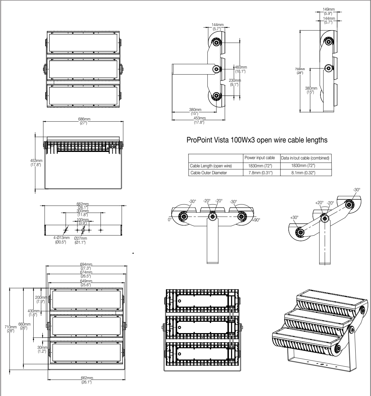
FIG.3: ProPoint Vista 3x100W
