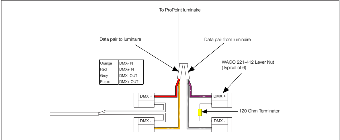
FIG.21: DMX Termination Detail
