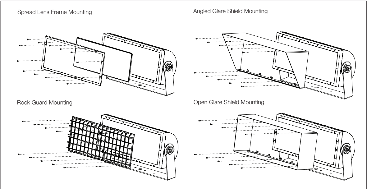
FIG.20: Accessories Mounting
