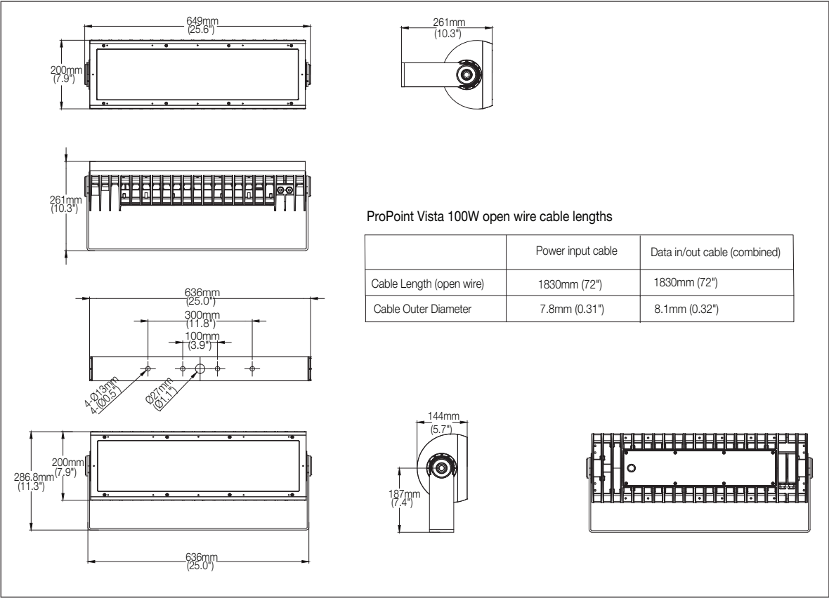
FIG.1: ProPoint Vista 1x100W
