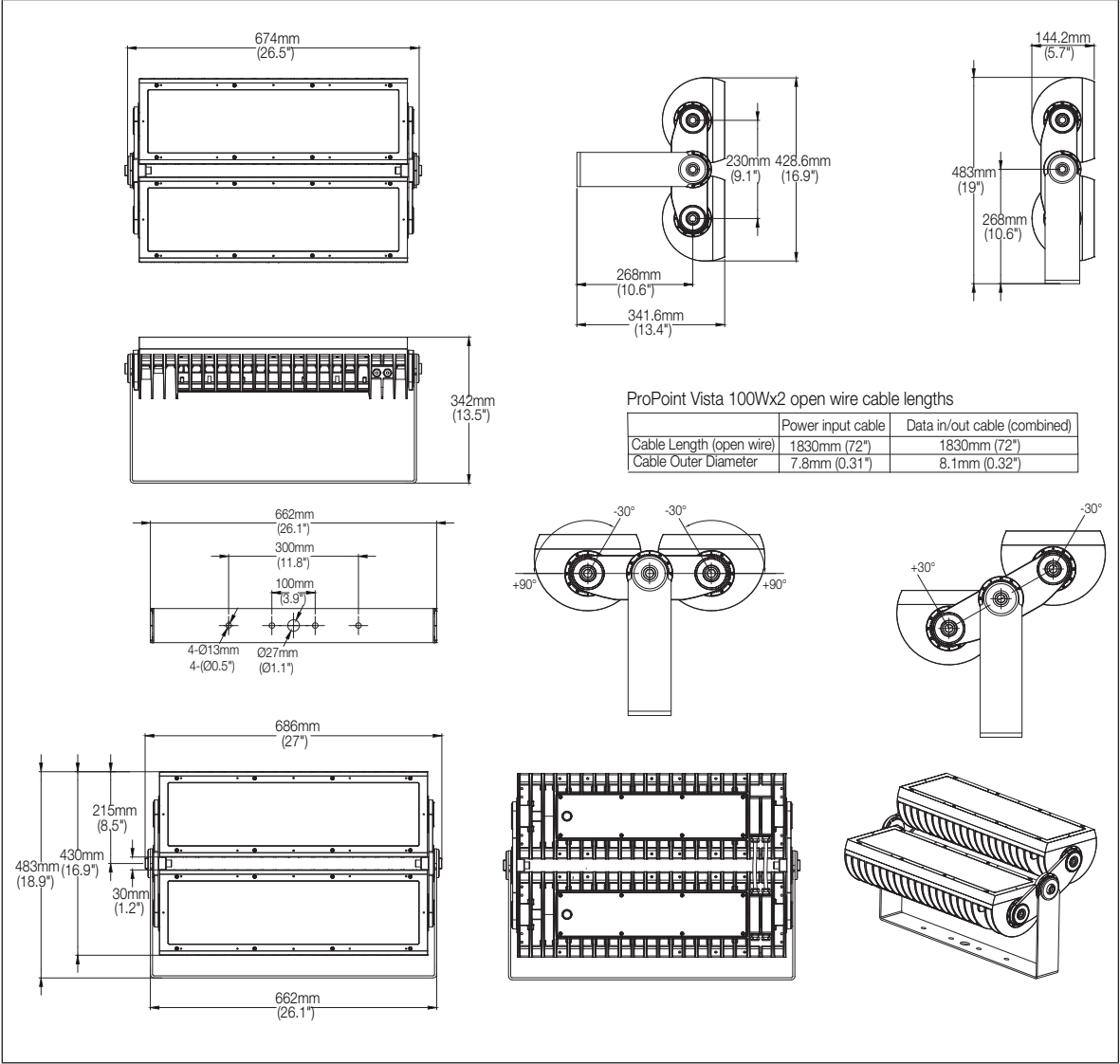
FIG.2: ProPoint Vista 2x100W
