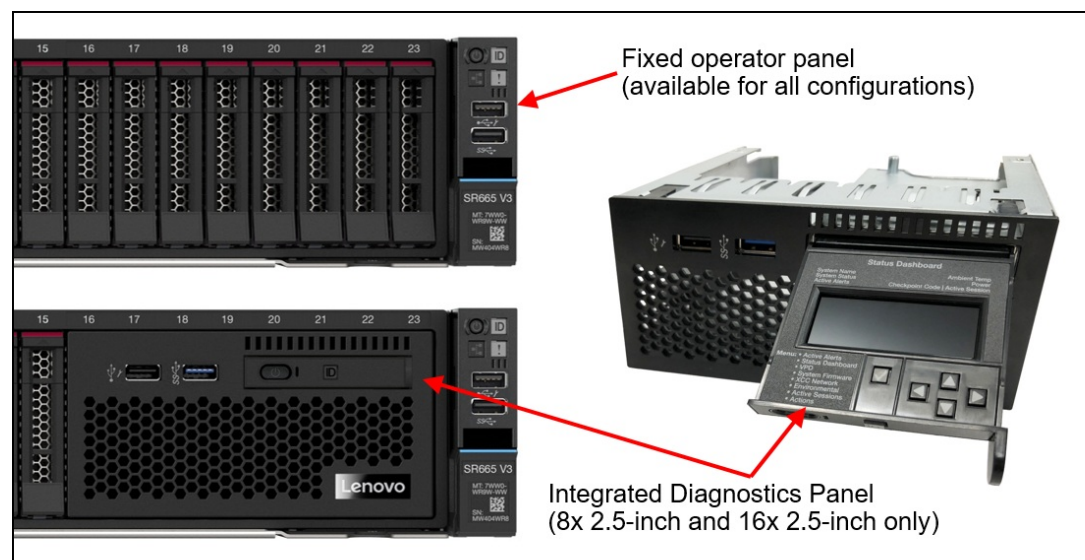
Figure 21. Operator panel choices for the 8x 2.5-inch drive bay configuration
