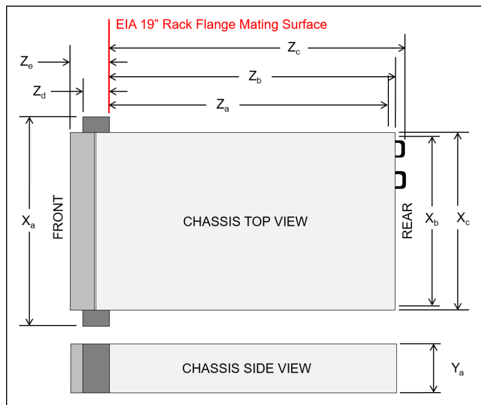
Figure 25. Server dimensions
