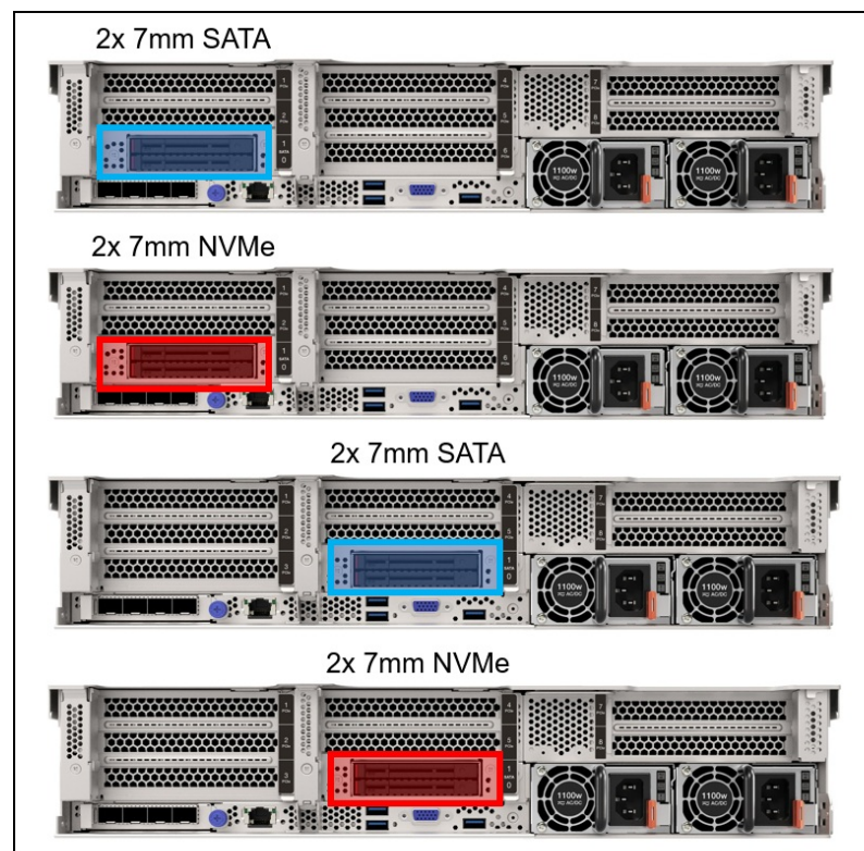
Figure 13. Rear 7mm drive bay configurations
