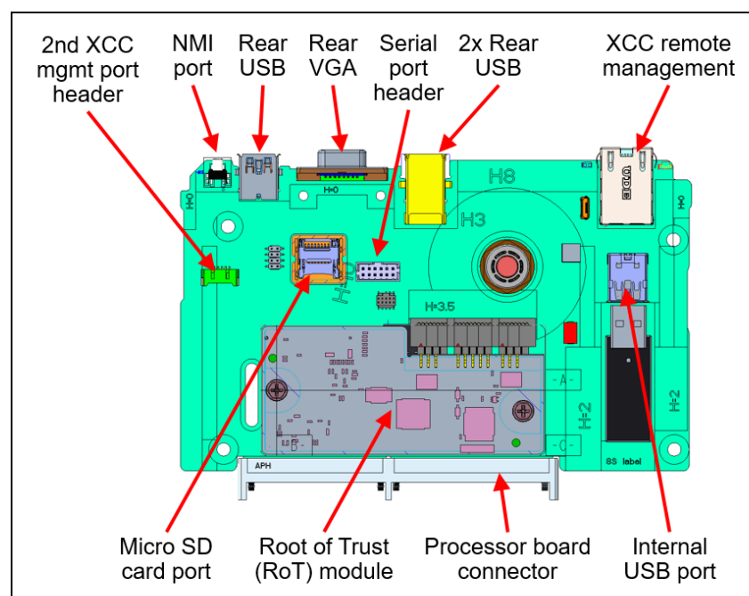
Figure 19. System I/O Board
