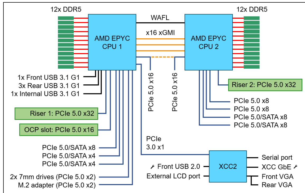
Figure 5. SR665 V3 system architectural block diagram
