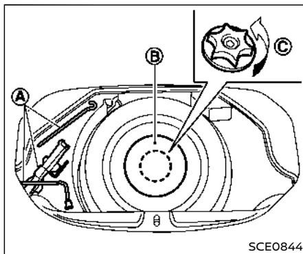
Without subwoofer
