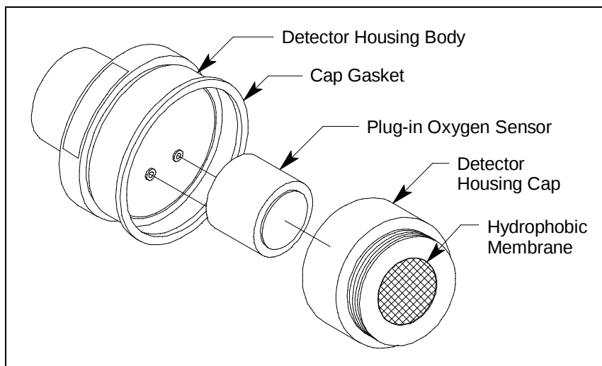
Figure 2: 65-2494RK Oxygen Detector Component Location
