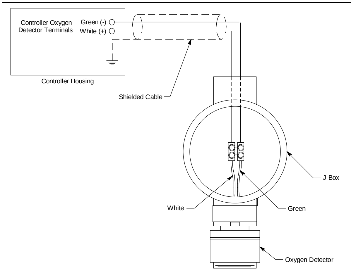
Figure 4: Wiring the Oxygen Detector to a Controller
