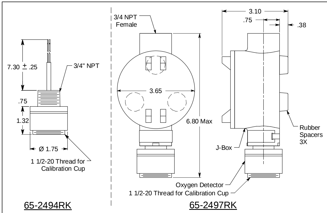
Figure 3: Outline & Mounting Dimensions, 65-2494RK & 65-2497RK
