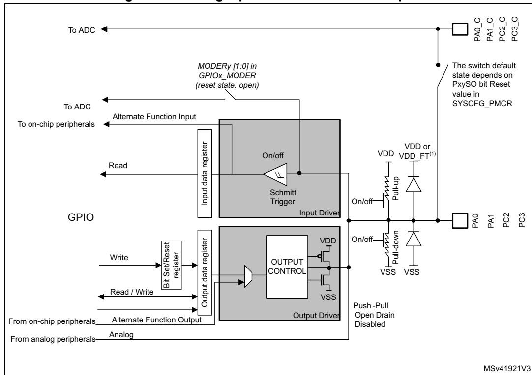
Figure 76. Analog inputs connected to ADC inputs
