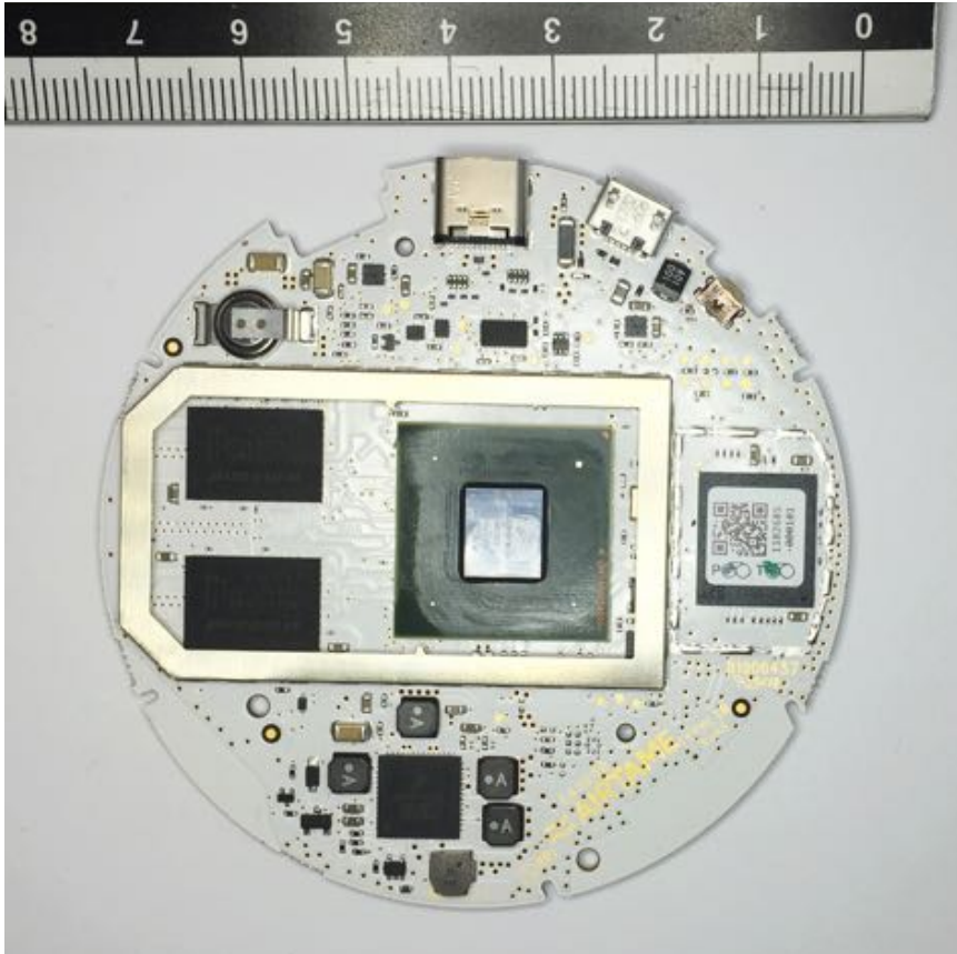
Top side without RF screen
