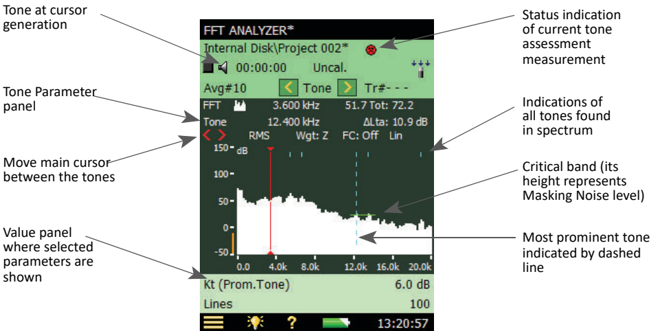
Fig. 7.5 Typical FFT spectrum display, showing the various fields
