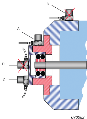
Fig. 3.2 Examples of different accelerometer mounting positions on the bearing of a drive shaft
