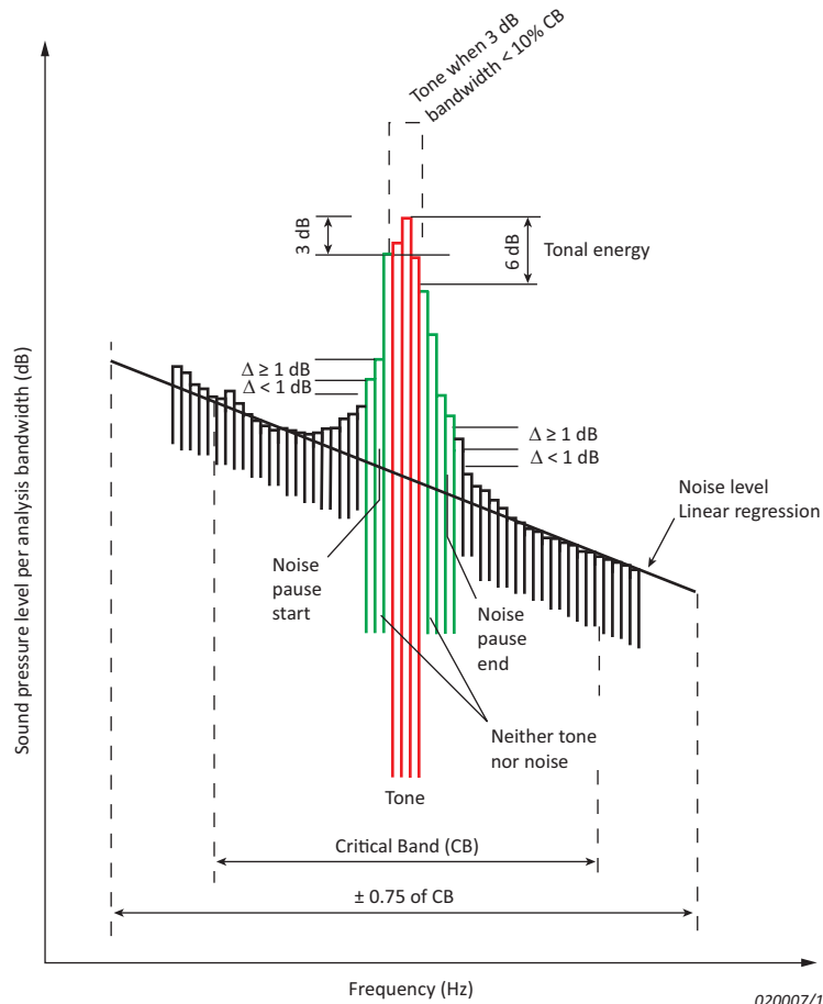
Fig. 7.1 Overview of terms related to FFT-based tone assessment
