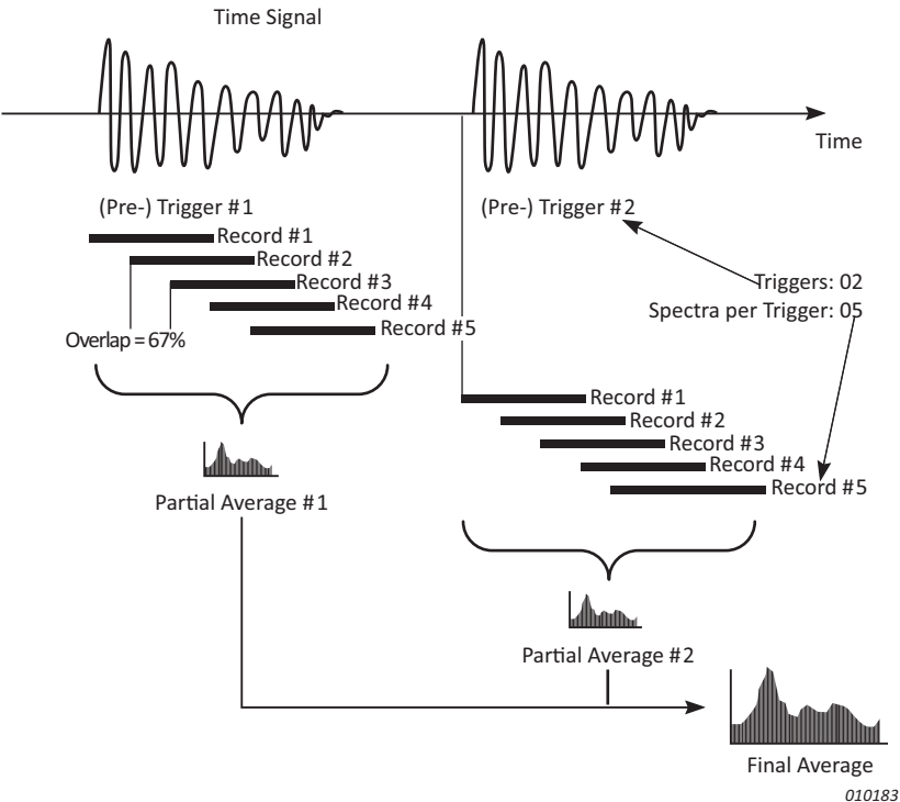
Fig. 5.14 Graphical explanation of what happens to records when measuring triggered, continuous signals using the set up described in section 5.3.2
