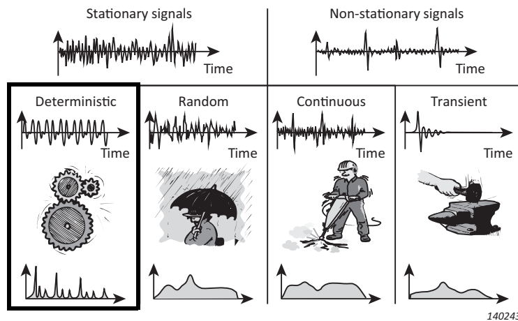
Fig. 6.1 Deterministic signals
