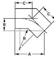
45° Mitered
