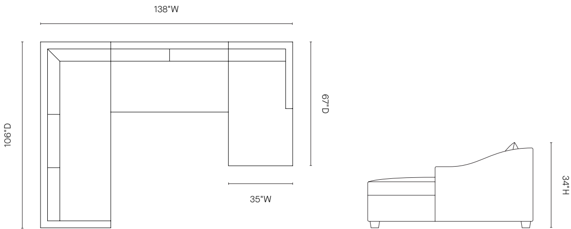
Chaise Left or Chaise Right: 138" x 106"
