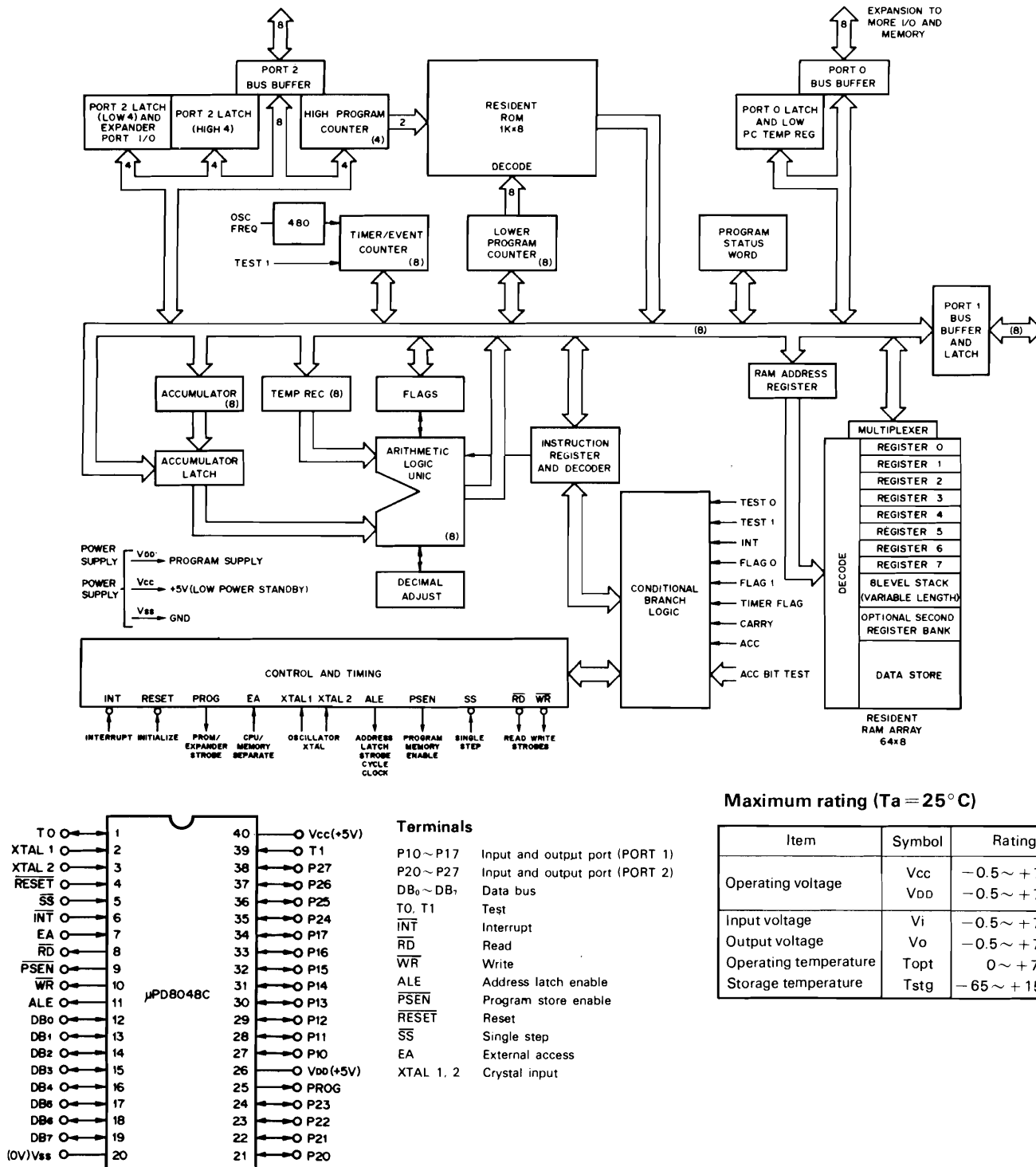
Fig. 13 \mu PD8048C-155 (DIGITAL UNIT, IC11)
