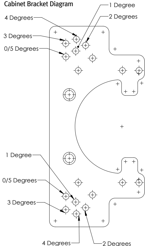
Cabinet Bracket Diagram
