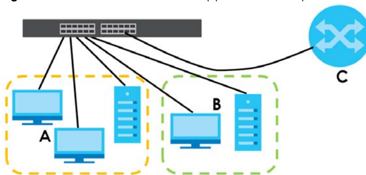
Figure 110 Protocol Based VLAN Application Example
