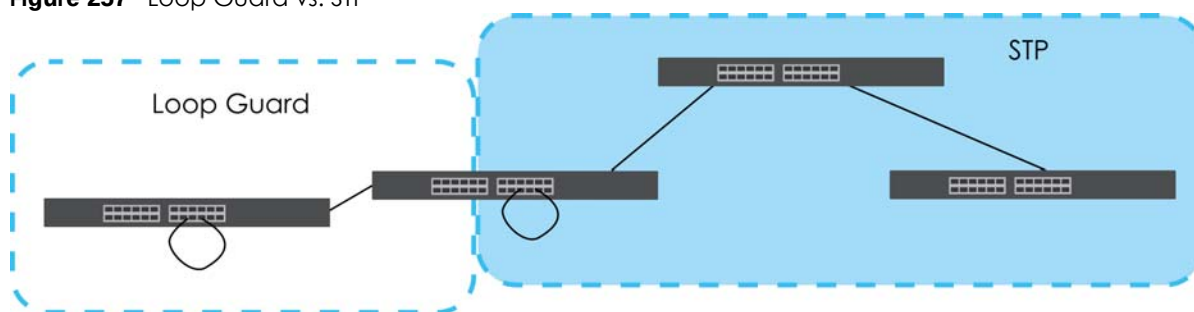
Figure 257 Loop Guard vs. STP
