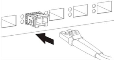
Figure 13 Connecting the Fiber Cables
