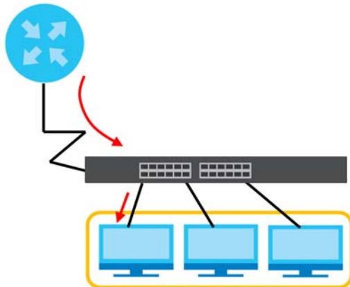
Figure 123 Static Multicast Forwarding to Multiple Ports
