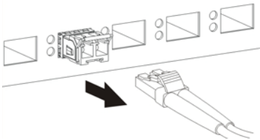
Figure 15 Opening the Transceiver's Latch Example
