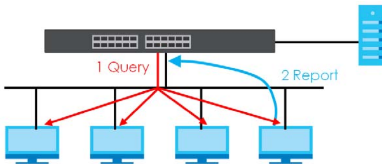
Figure 367 IGMP Version 1 Example
