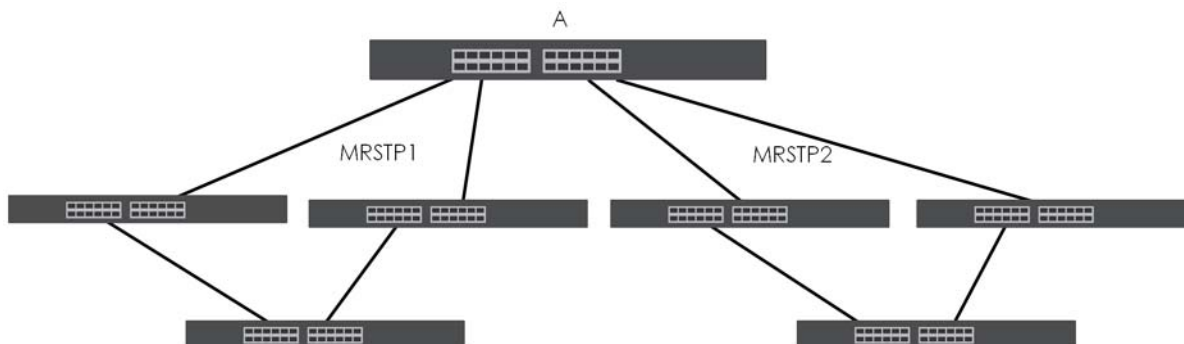
Figure 126 MRSTP Network Example
