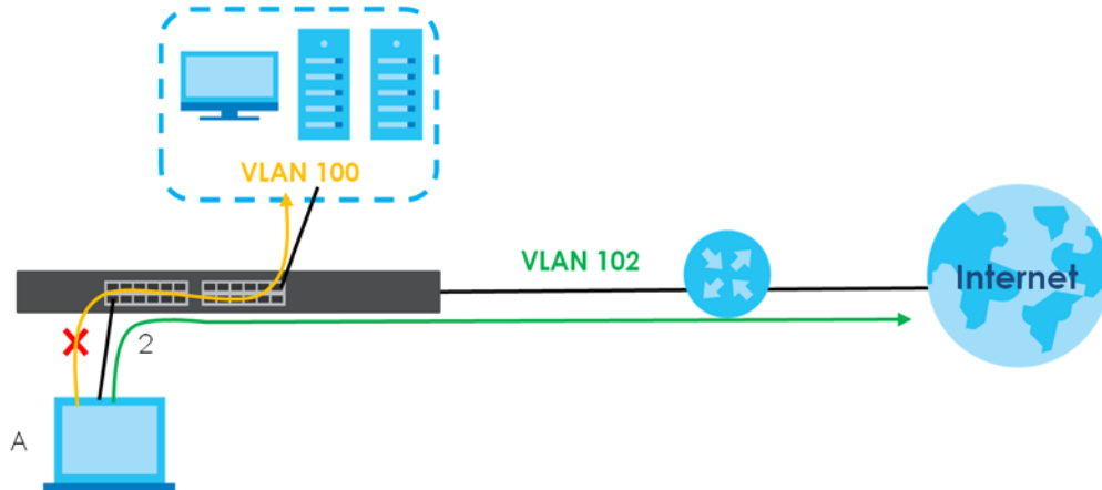
Figure 174 Guest VLAN Example
