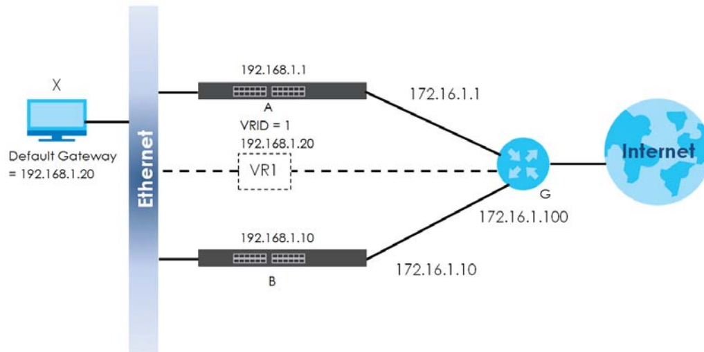
Figure 403 VRRP Configuration Example: One Virtual Router Network
