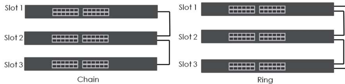
Figure 90 Stacking Topology
