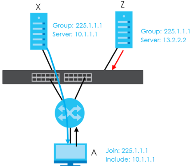
Figure 369 IGMP Version 3 Example
