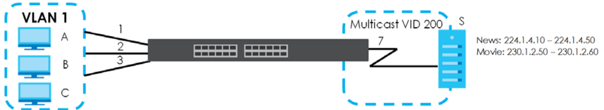
Figure 219 MVR Configuration Example
