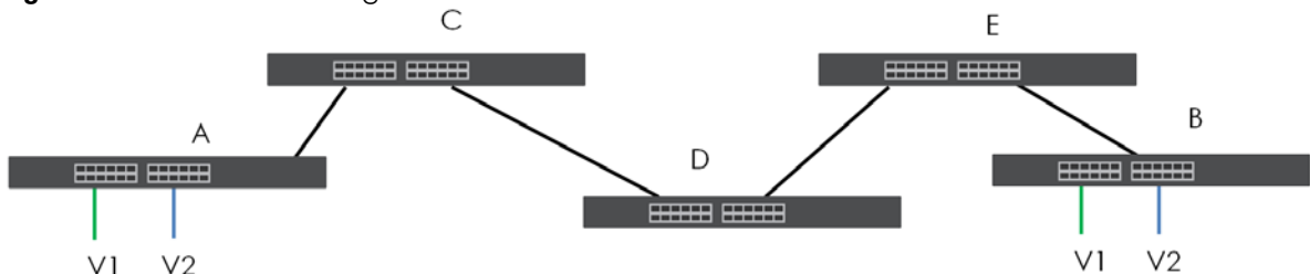
Figure 97 Port VLAN Trunking
