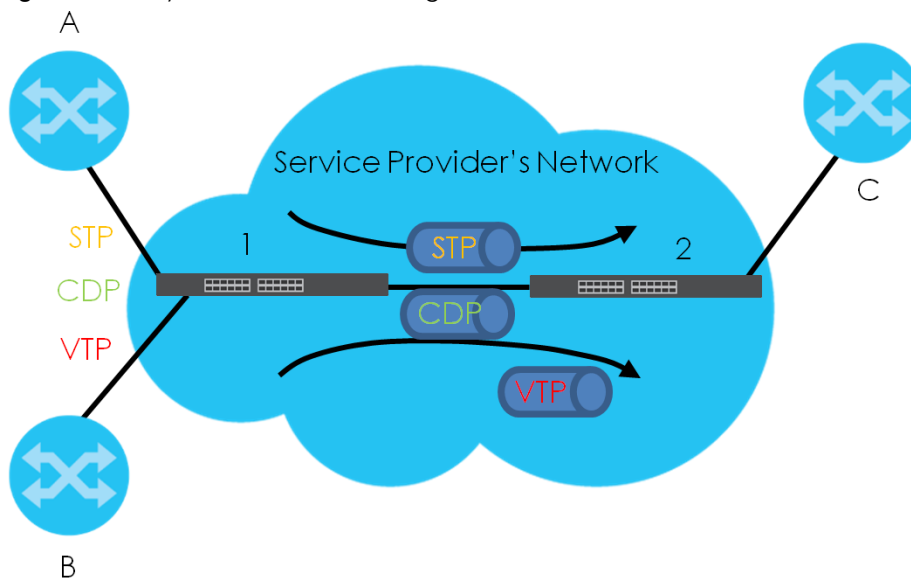
Figure 268 Layer 2 Protocol Tunneling Network Scenario
