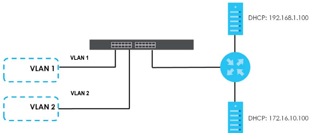
Figure 391 DHCP Relay for Two VLANs
