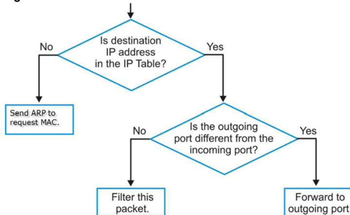
Figure 466 IP Table Flowchart
