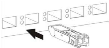
Figure 12 Transceiver Installation Example
