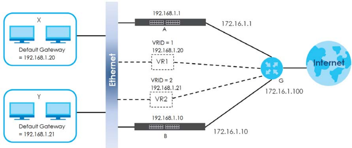
Figure 408 VRRP Configuration Example: Two Virtual Router Network
