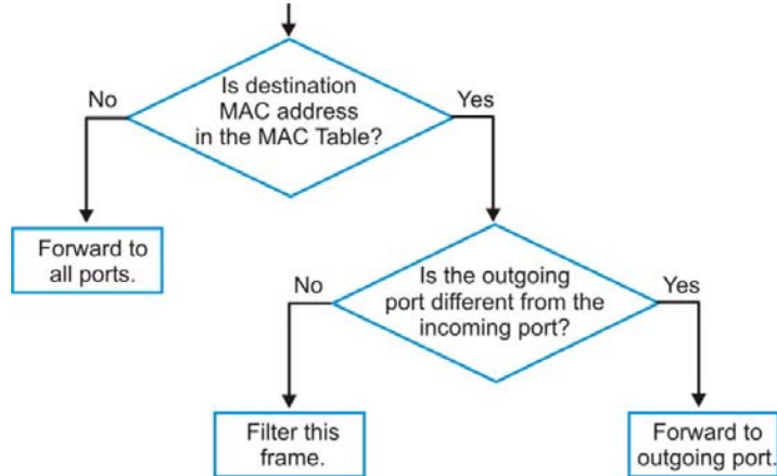
Figure 464 MAC Table Flowchart
