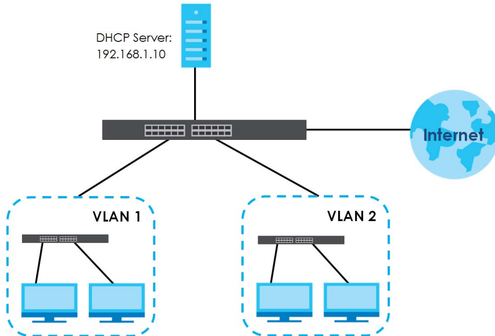
Figure 387 Global DHCP Relay Network Example
