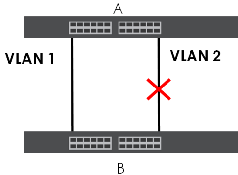
Figure 143 STP/RSTP Network Example
