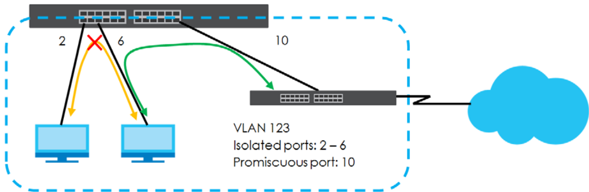
Figure 290 VLAN Isolation Example
