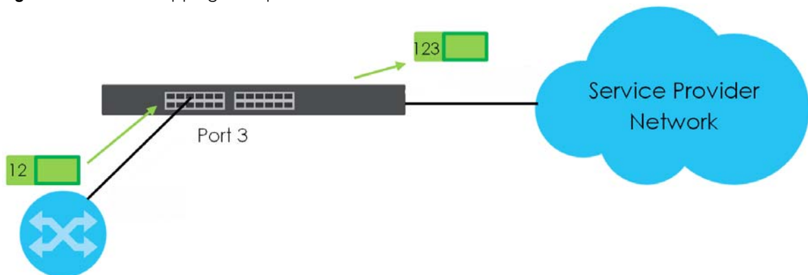
Figure 263 VLAN Mapping Example
