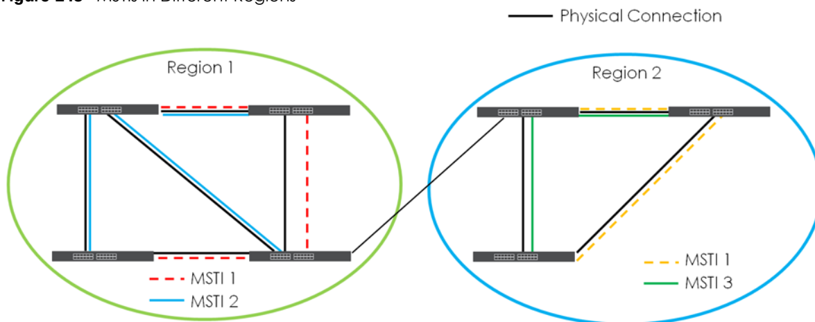
Figure 145 MSTIs in Different Regions
