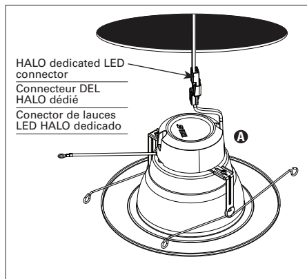
Figure 6. LED Connection
