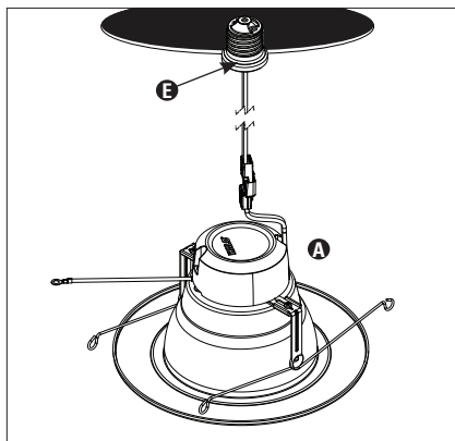
Figure 5. Retrofit Connection
