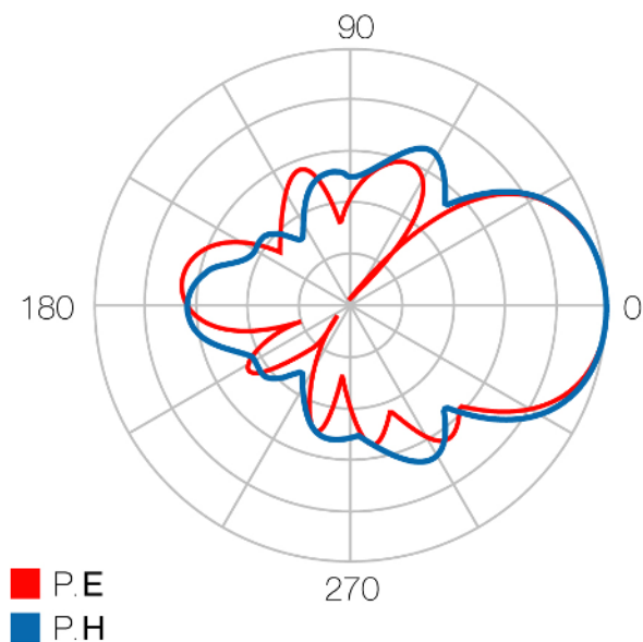
Radiation pattern
