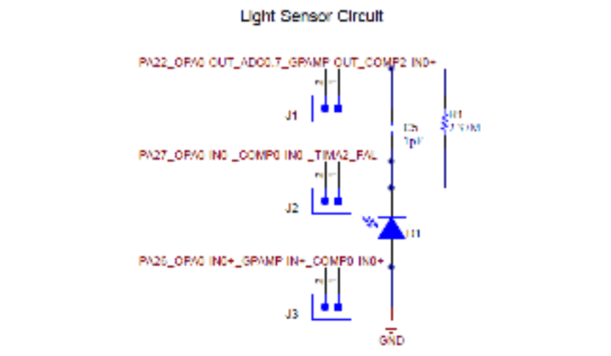
Figure 2-9. Light Sensor Circuit
