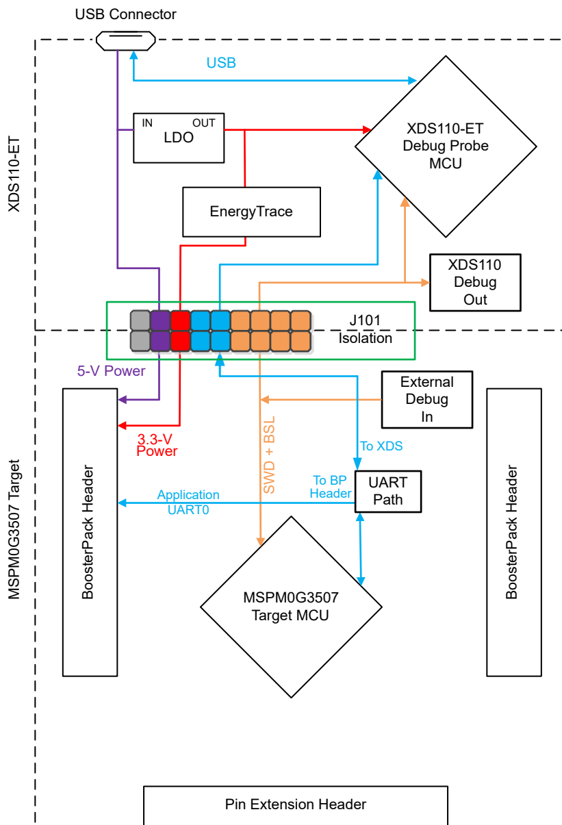
Figure 2-5. Isolation Jumper Block
