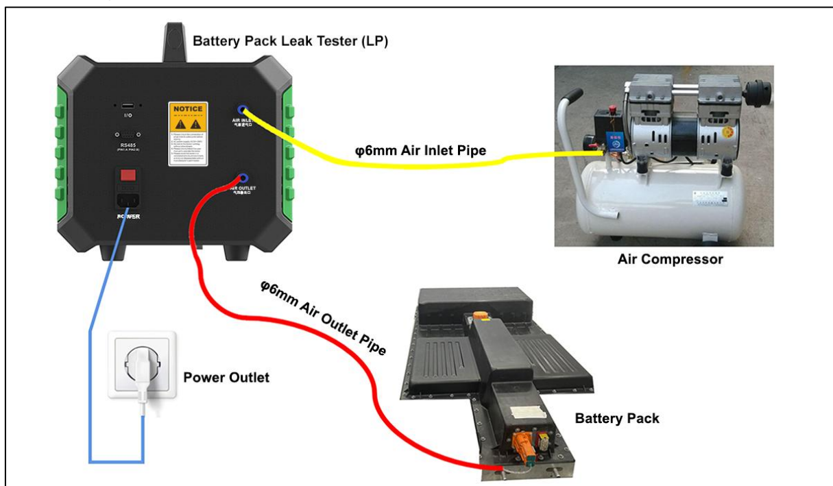
Connecting Diagram
