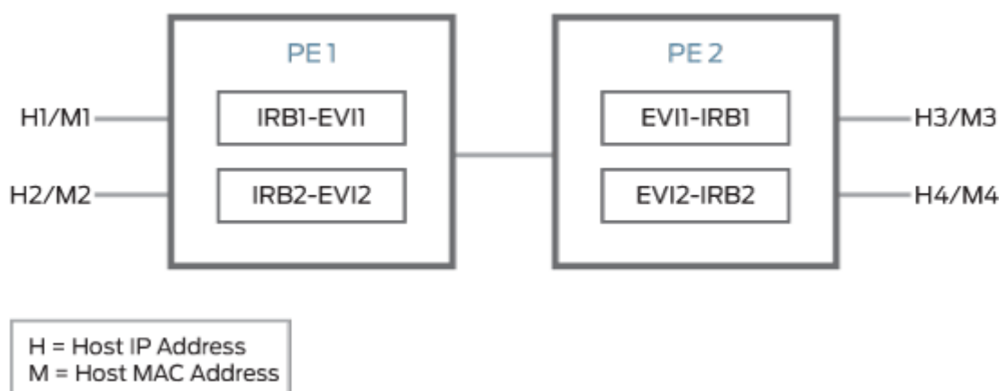
Figure 136: Inter-Subnet Traffic Forwarding
