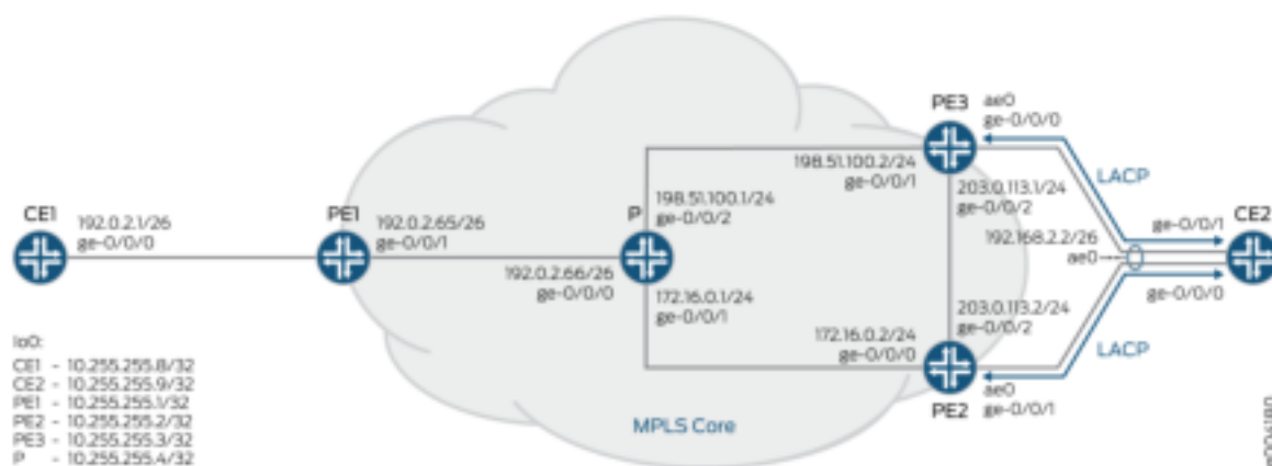
Figure 28: LACP Support in EVPN Active-Active Multihoming
