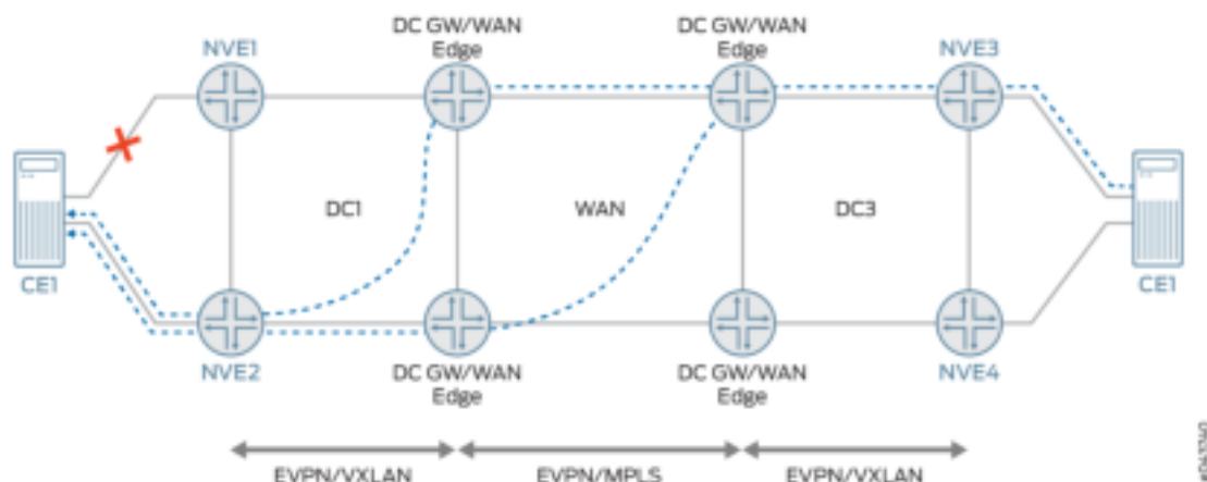
Figure 172: Load Balancing Among Redundant DC GW/WAN Edge Routers
