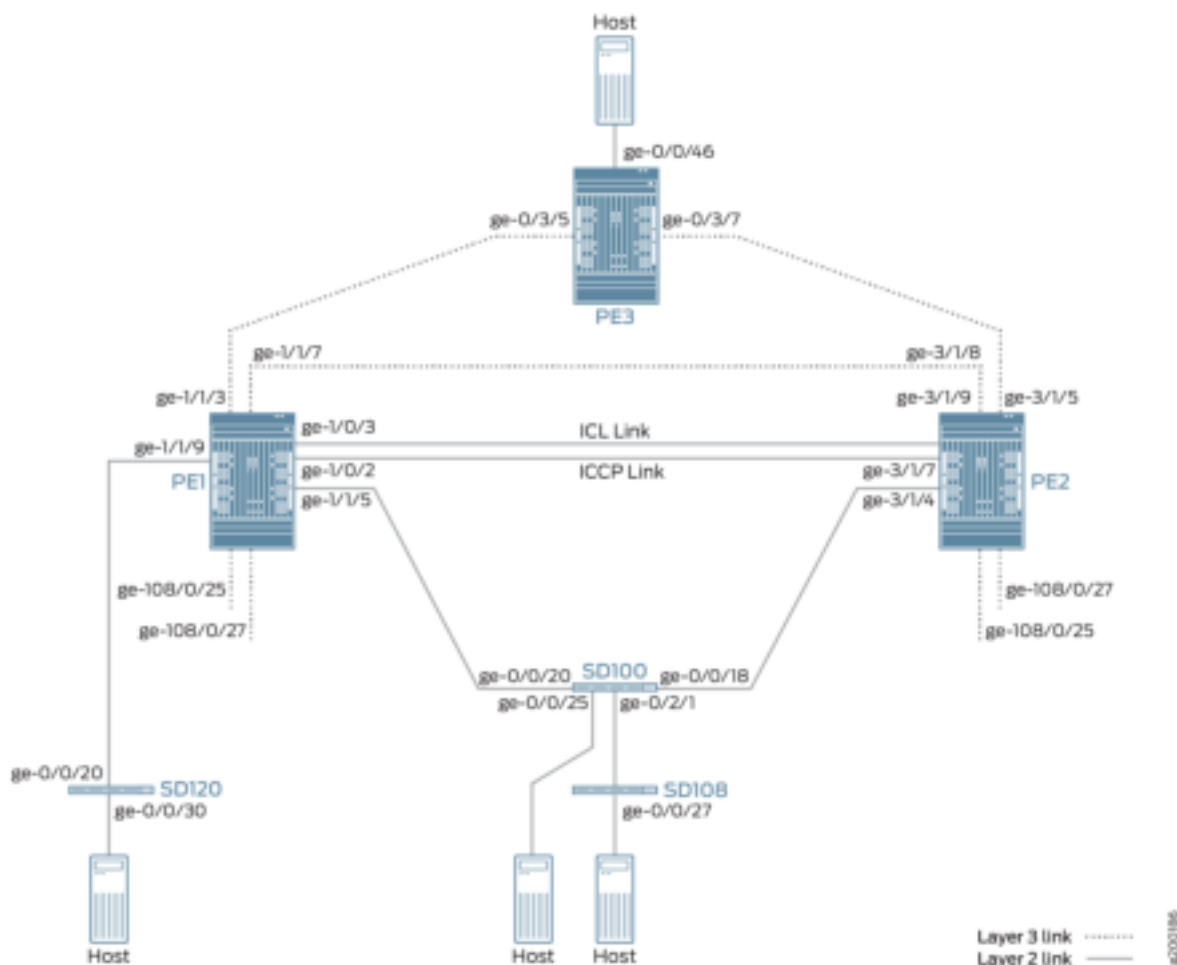
Figure 178: EVPN-MPLS Interworking with Junos Fusion Enterprise
