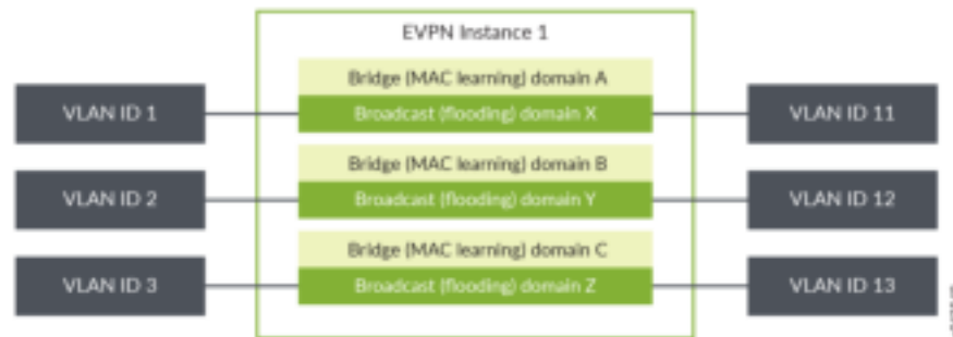
Figure 130: VLAN-Aware Bundle Service
