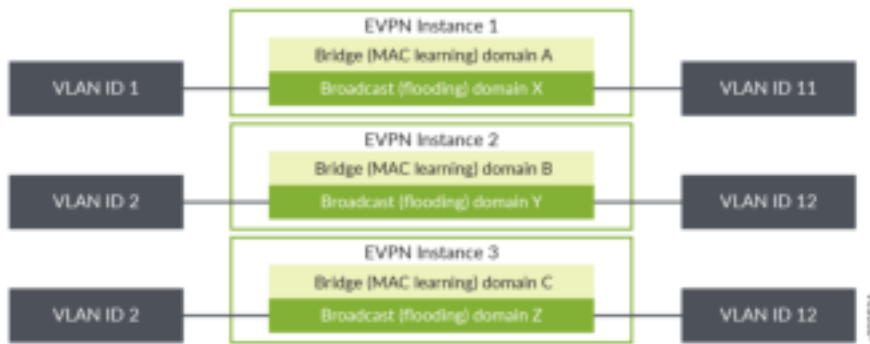
Figure 128: VLAN-Based Service
