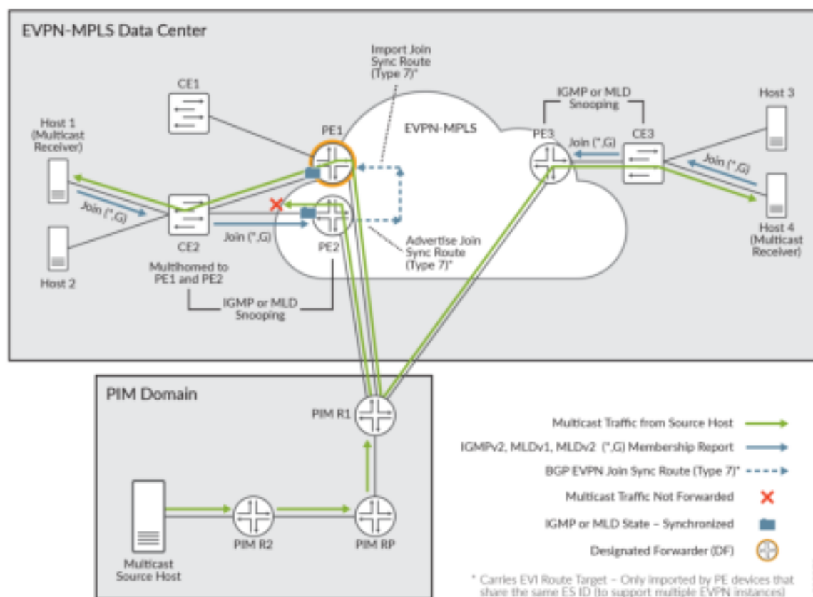
Figure 140: Multicast Forwarding for Multihomed Receivers in EVPN-MPLS on ACX Series Routers
