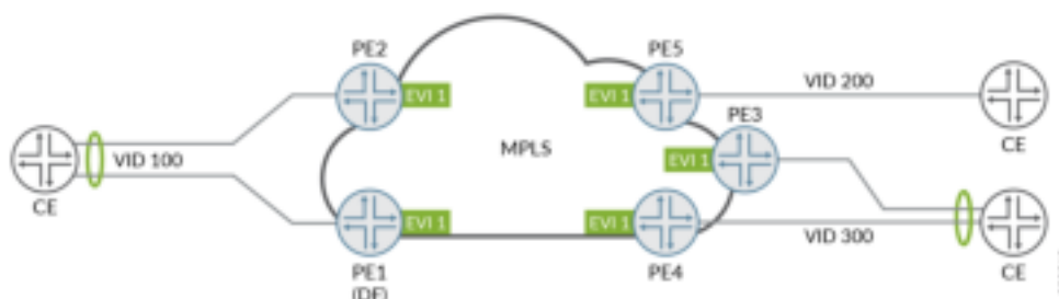
Figure 132: Multiple VIDs with VLAN Translation
