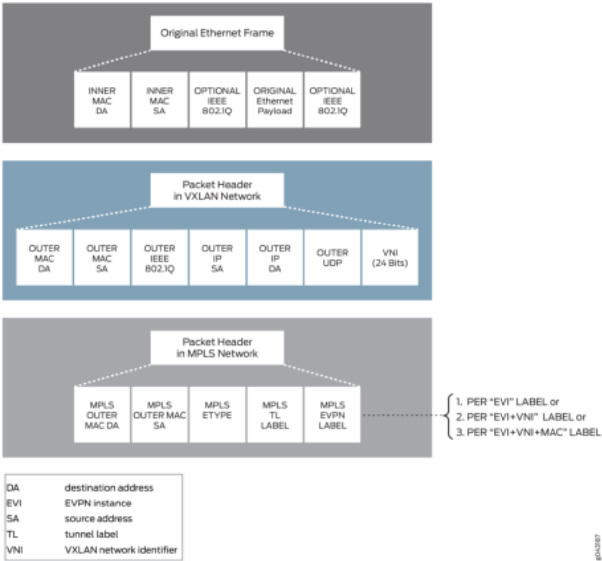
Figure 44: EVPN-VXLAN Packet Format
