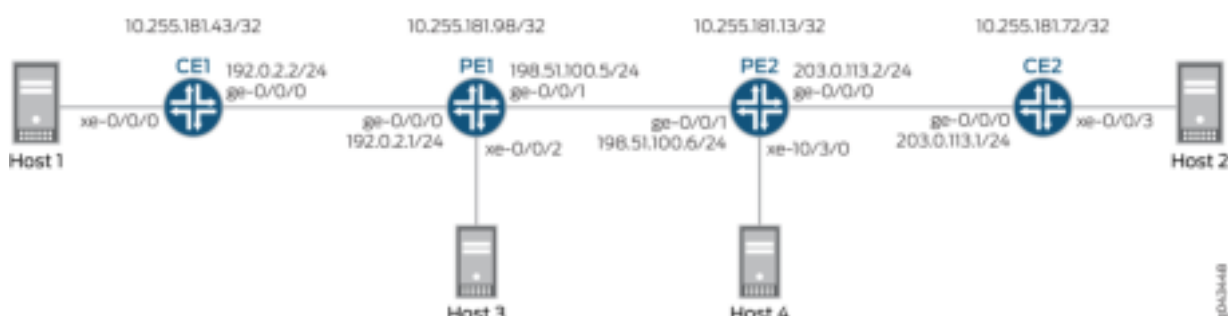
Figure 169: VXLAN Data Center Interconnect Using EVPN
