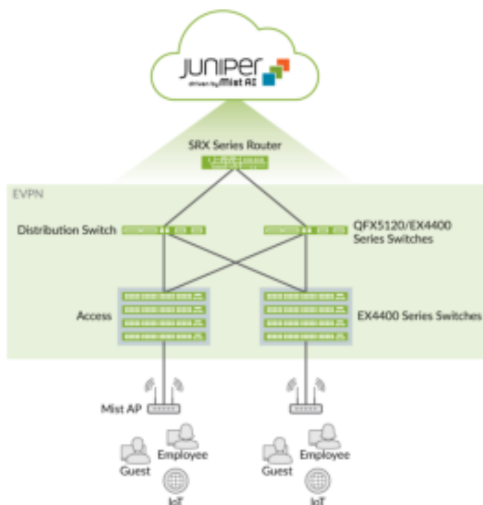
Figure 61: VXLAN GBP on an EX4400 Switch
