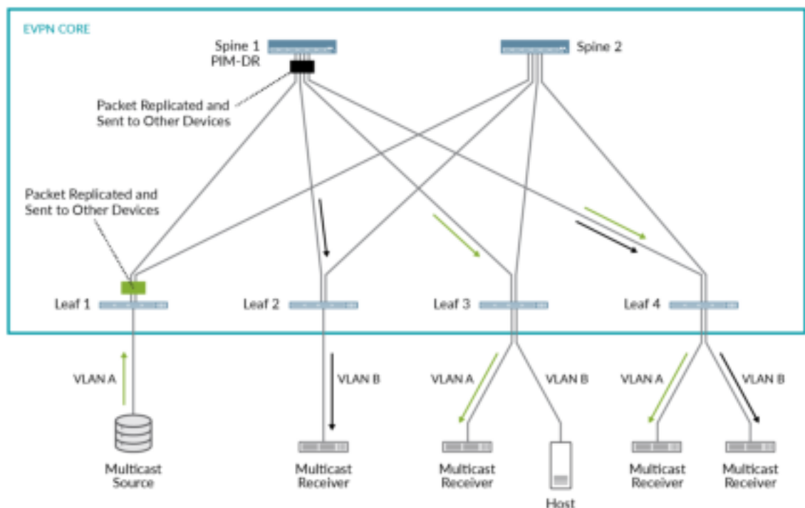
Figure 94: Selective Multicast Forwarding in a Centrally-Routed EVPN-VXLAN Network
