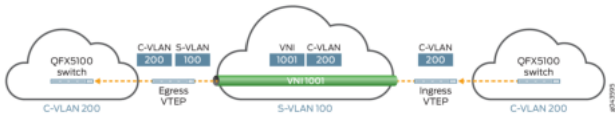
Figure 116: Mapping a Range of C-VLANs to an S-VLAN
