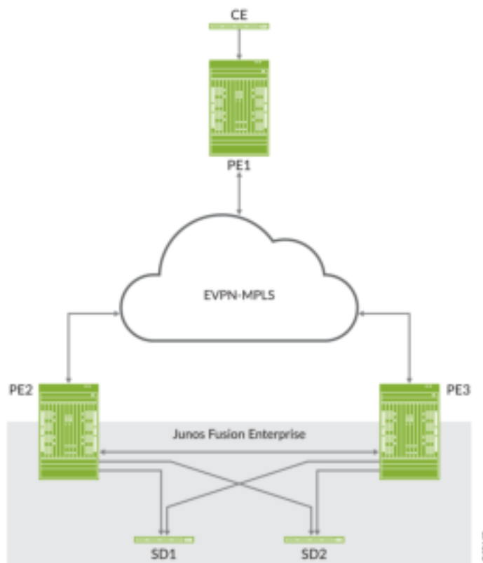
Figure 176: EVPN-MPLS Interworking with Junos Fusion Enterprise
