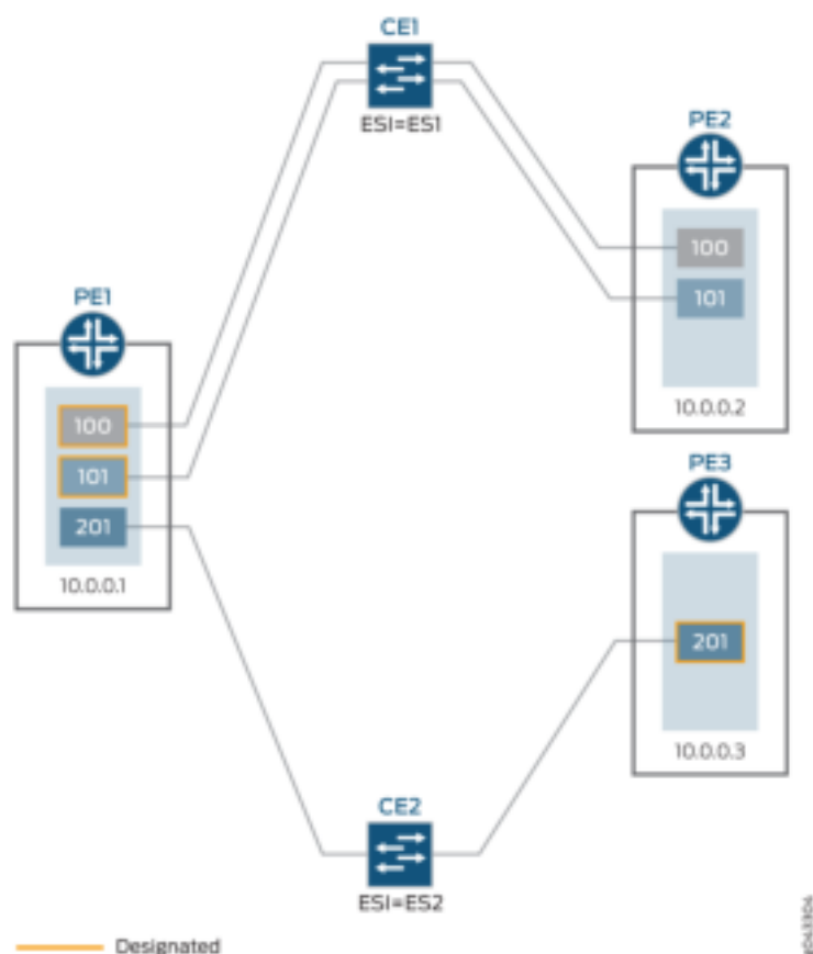
Figure 46: Designated Forwarder Election Topology
