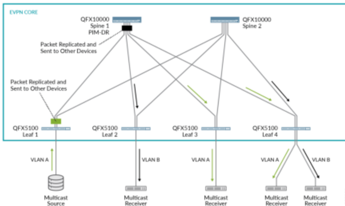
Figure 85: Centrally-Routed Bridging Overlay
