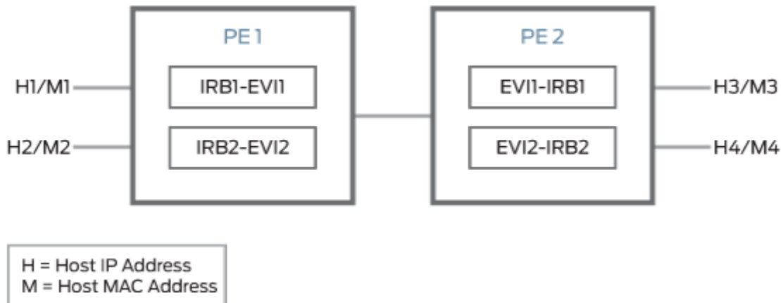
Figure 135: Inter-Subnet Traffic Forwarding
