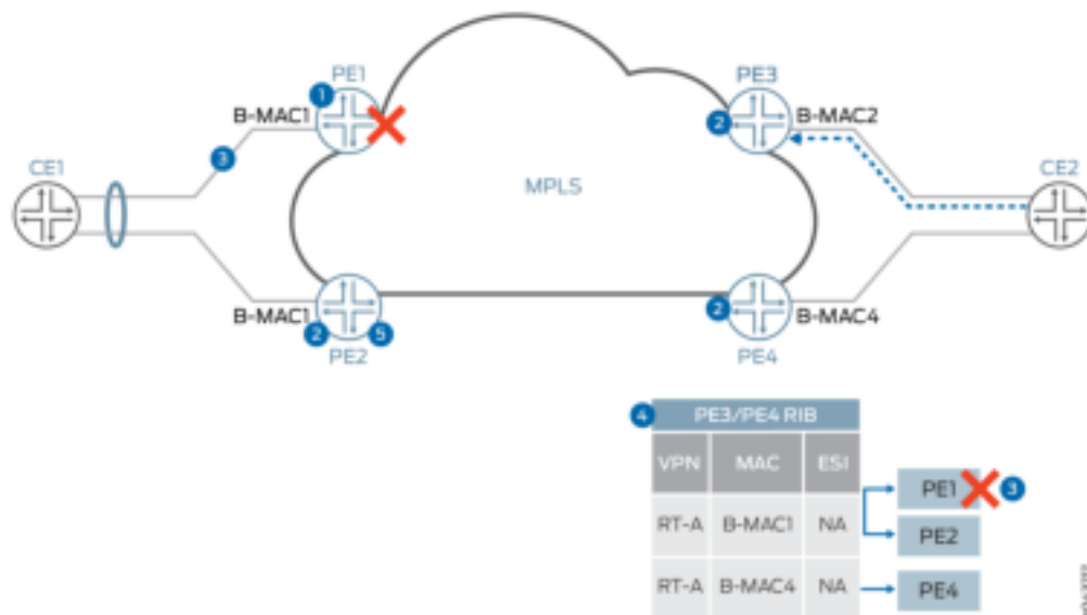
Figure 194: PBB-EVPN Core Failure
