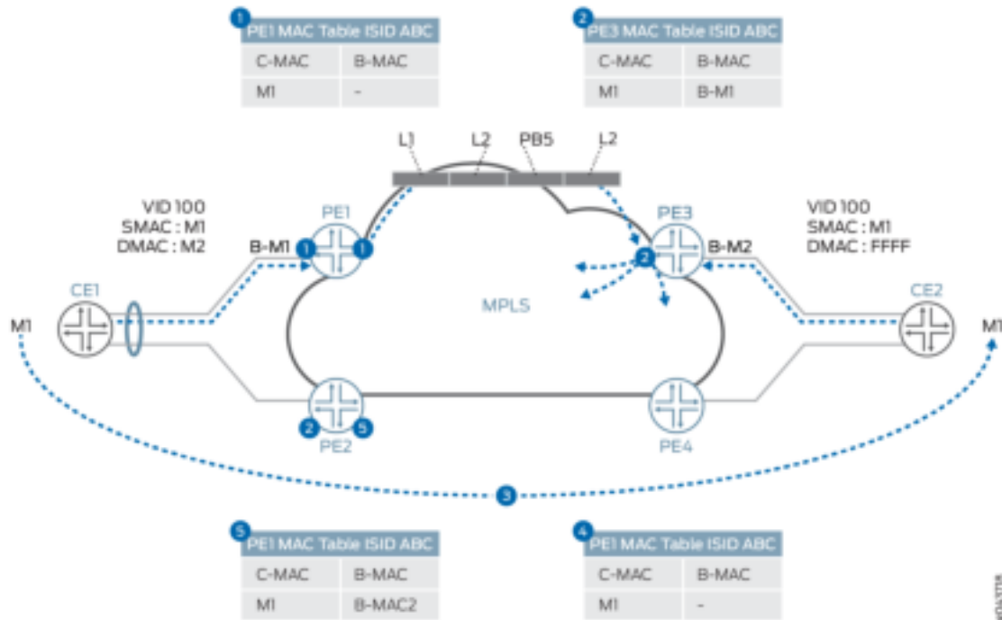
Figure 191: PBB-EVPN MAC Mobility Handling
