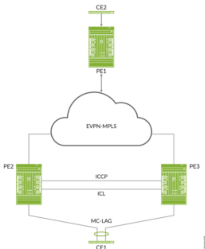
Figure 177: EVPN-MPLS Interworking with MC-LAG
