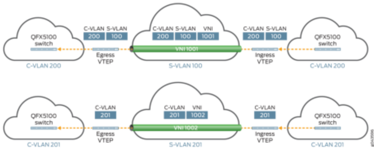
Figure 117: Retaining S-VLAN and C-VLAN Tags
