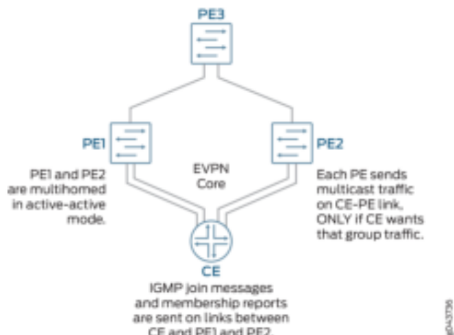
Figure 92: IGMP Snooping in an EVPN-VXLAN Environment
