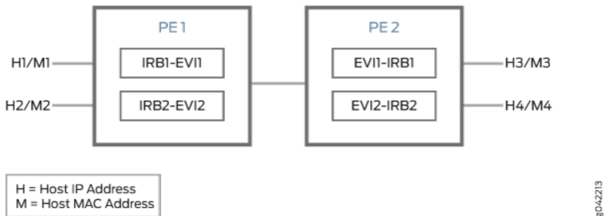
Figure 137: Inter-Subnet Traffic Forwarding
