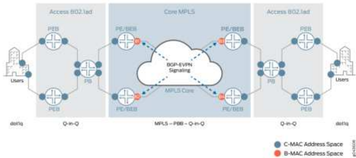
Figure 184: PBB-EVPN Integration
