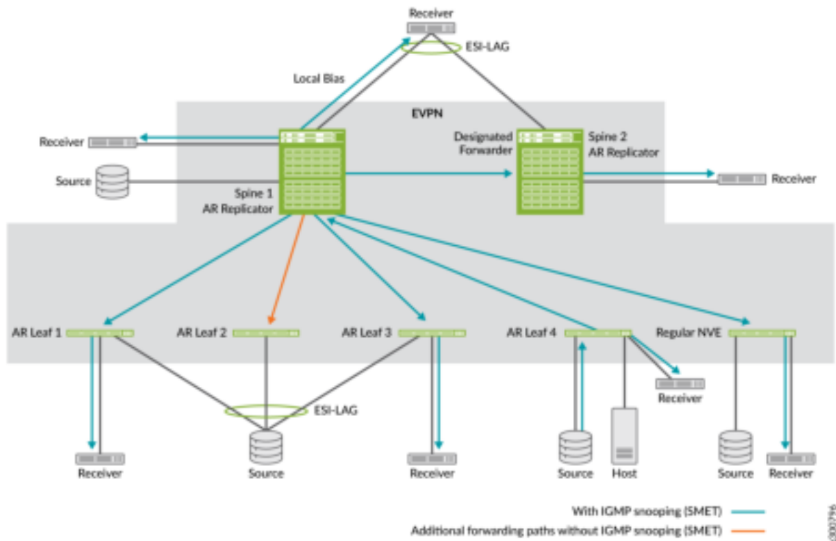
Figure 100: Source Traffic Ingress at an AR Leaf Device (Single-Homed Source)
