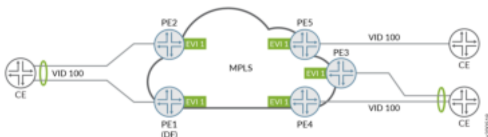
Figure 131: Single VID with no VLAN Translation
