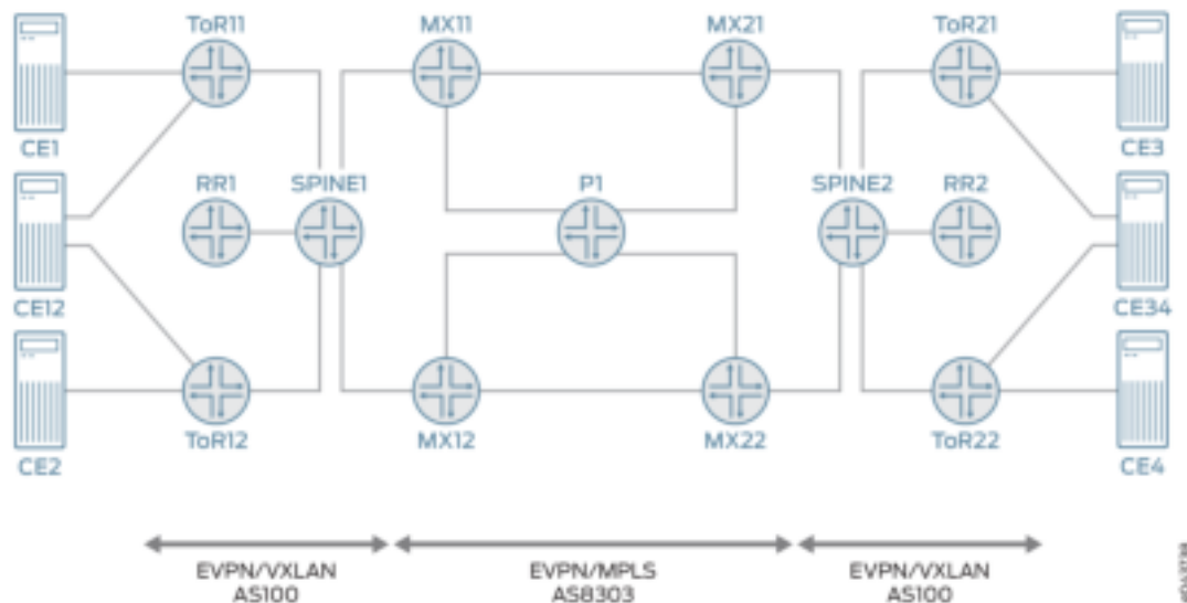
Figure 173: Data Center Network Design
