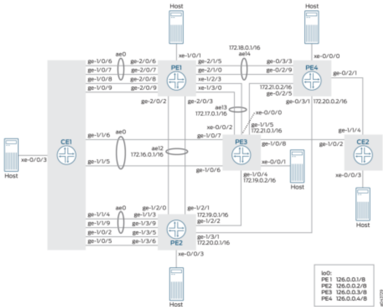
Figure 198: PBB with Active/Standby EVPN Multihoming
