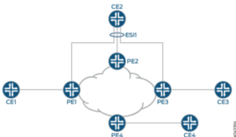
Figure 13: Active-Active EVPN Multihoming
