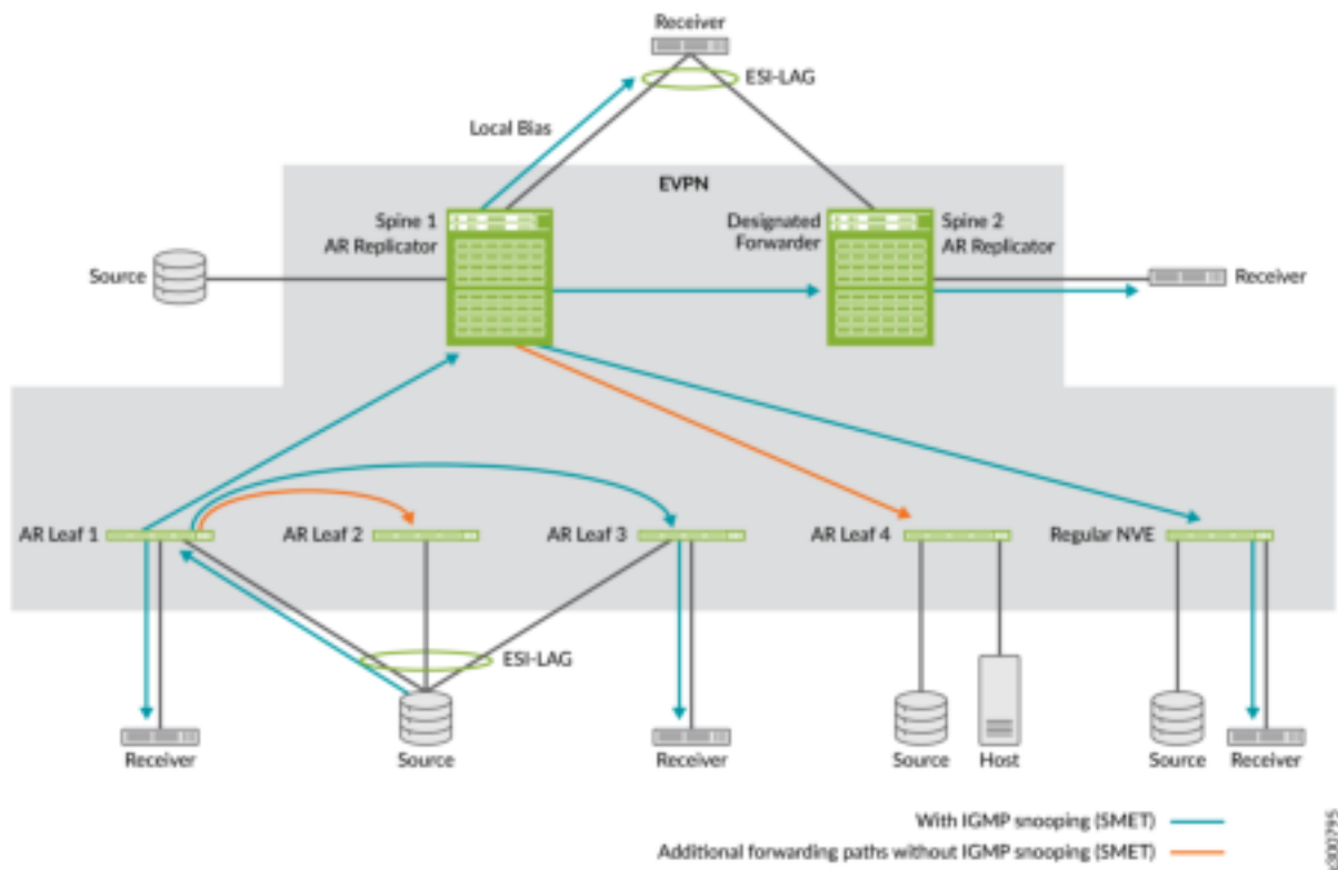
Figure 101: Source Traffic Ingress at an AR Leaf Device (Multihomed Source)
