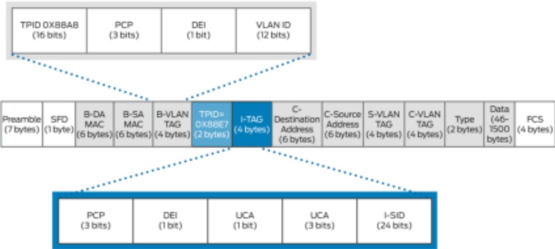
Figure 182: PBB Packet Format
