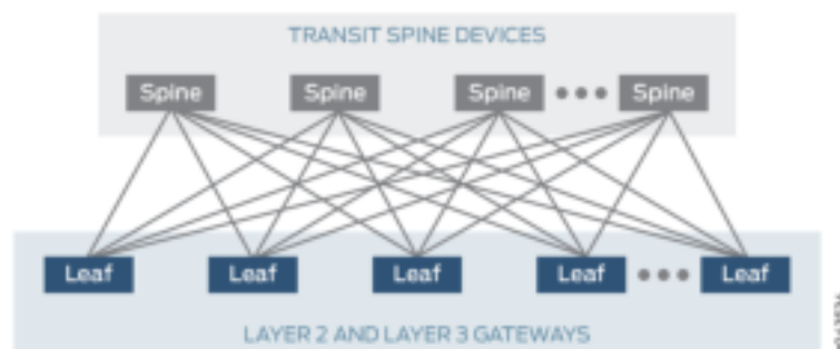
Figure 79: A 3-Stage (Leaf and Spine) Edge-Routing Bridging Architecture
