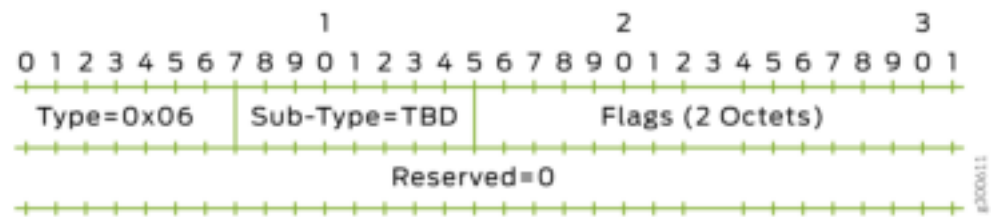
Figure 91: EVPN Multicast Flag Extended Community
