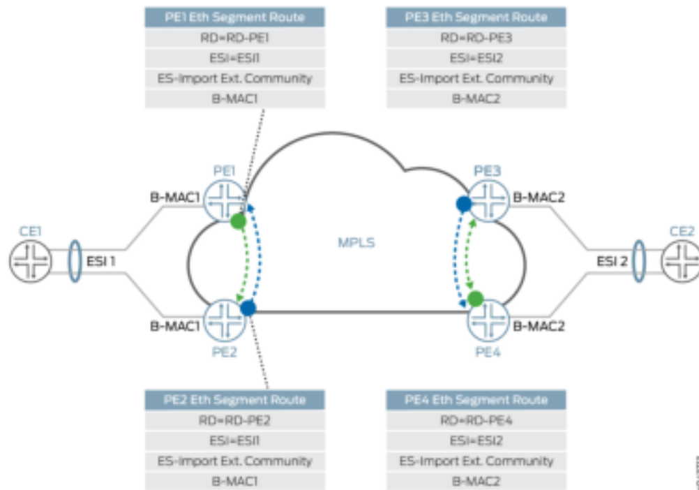
Figure 187: Ethernet Segment Discovery
