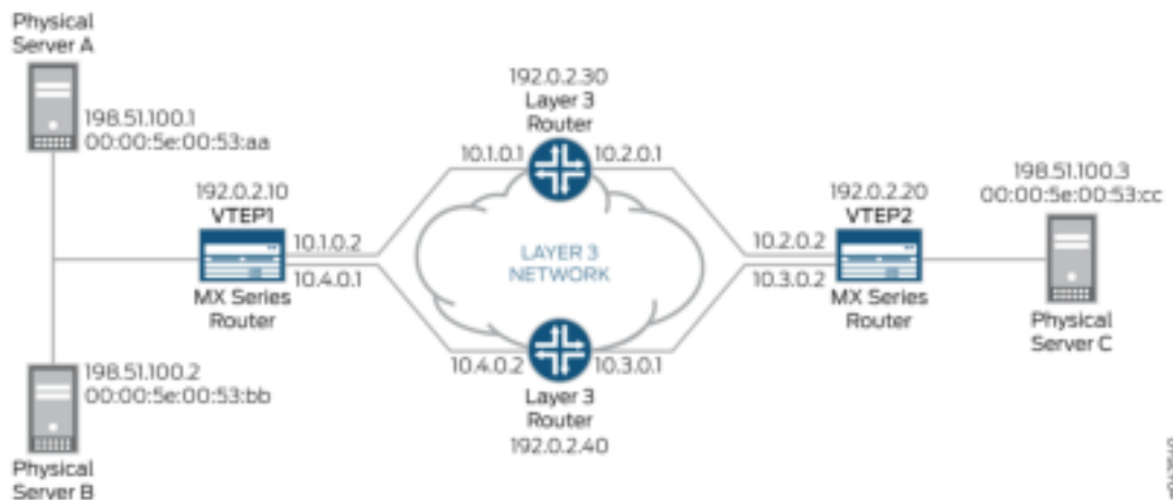
Figure 123: Using Overlay Ping and Traceroute to Troubleshoot a VXLAN
