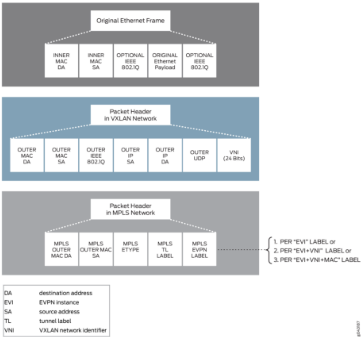
Figure 161: VXLAN-EVPN Packet Format
