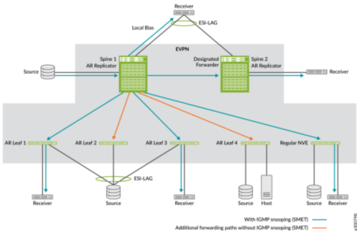
Figure 99: Multicast Source Traffic Ingress at an AR Replicator Device
