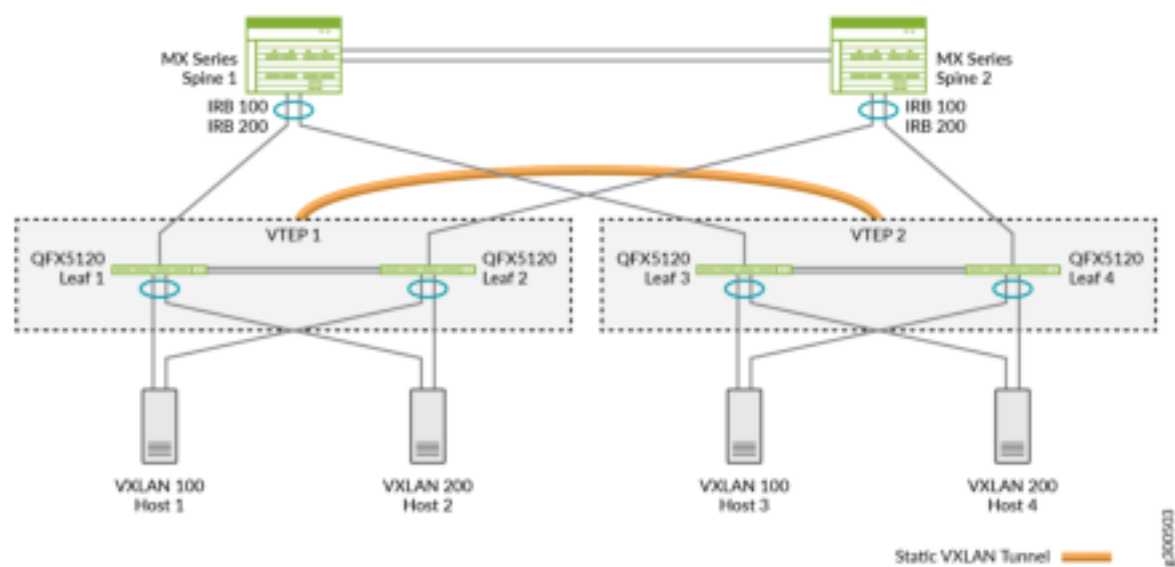
Figure 203: Sample MC-LAG Network with Static VXLAN
