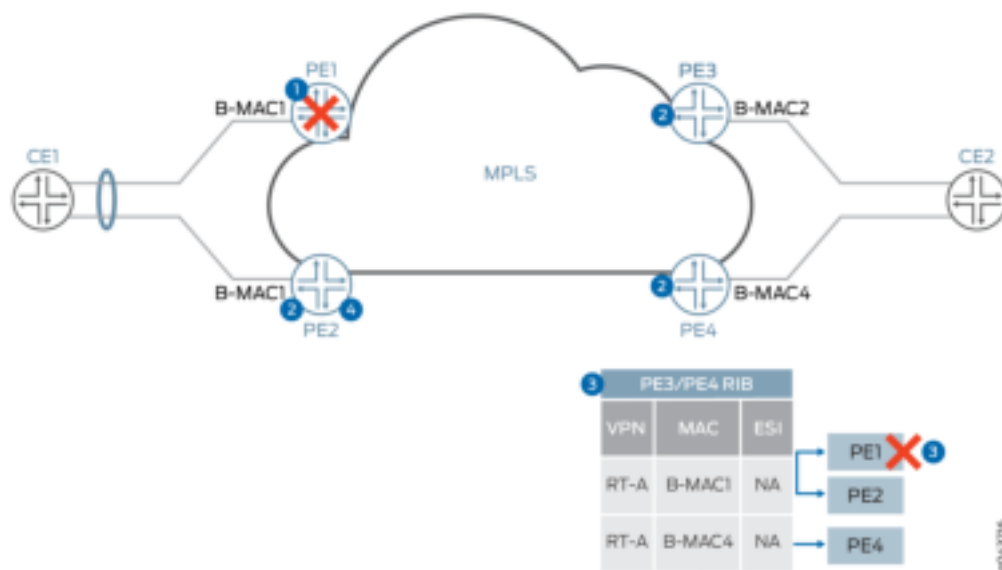
Figure 193: PBB-EVPN Node Failure
