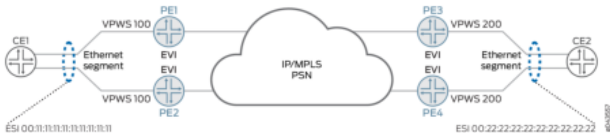
Figure 145: VPWS in EVPN
