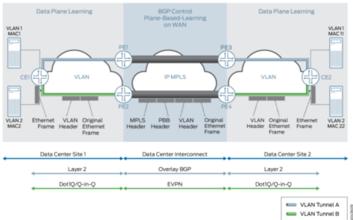
Figure 185: PBB-EVPN Control Plane Handling
