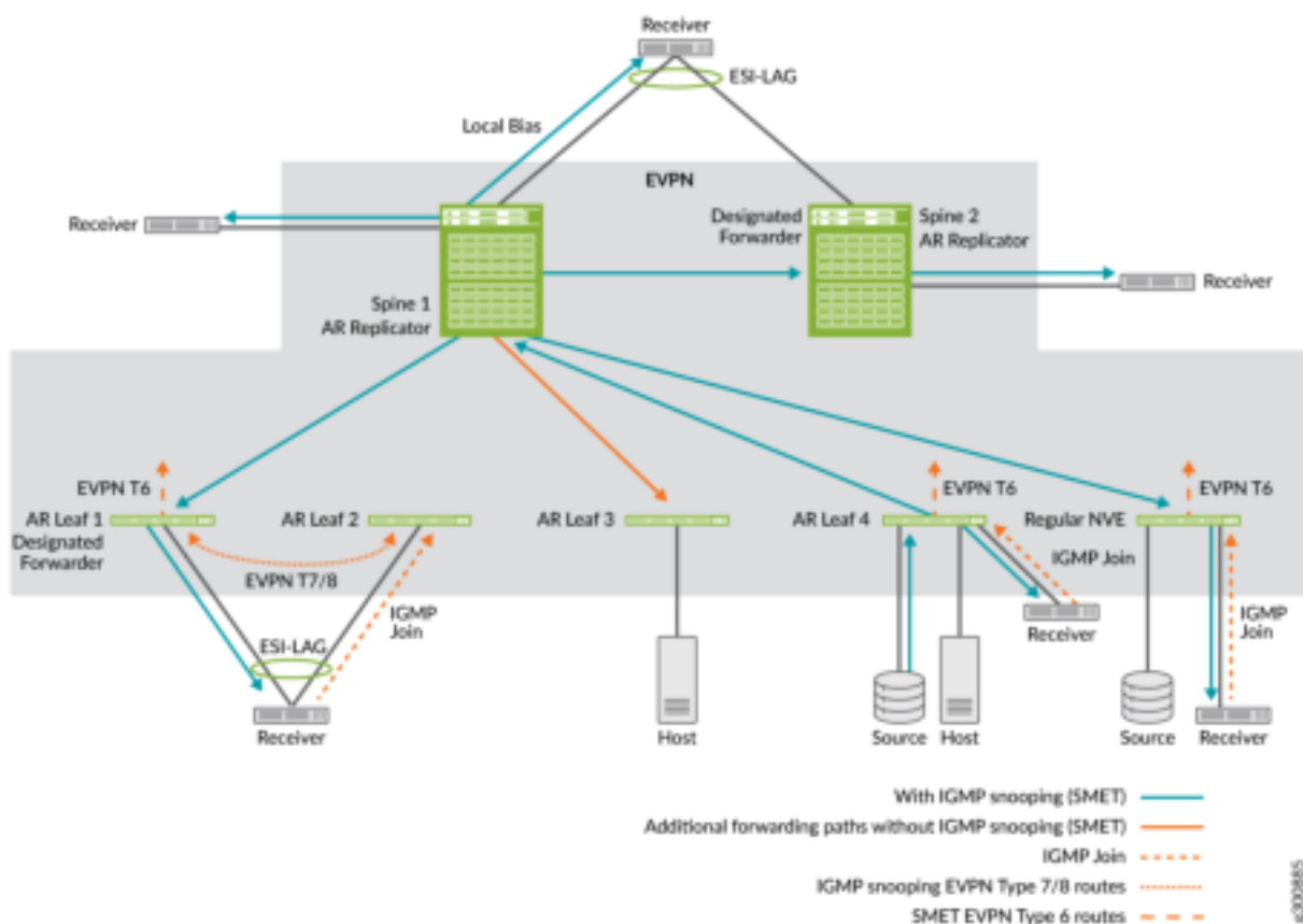
Figure 95: AR Traffic Flow
