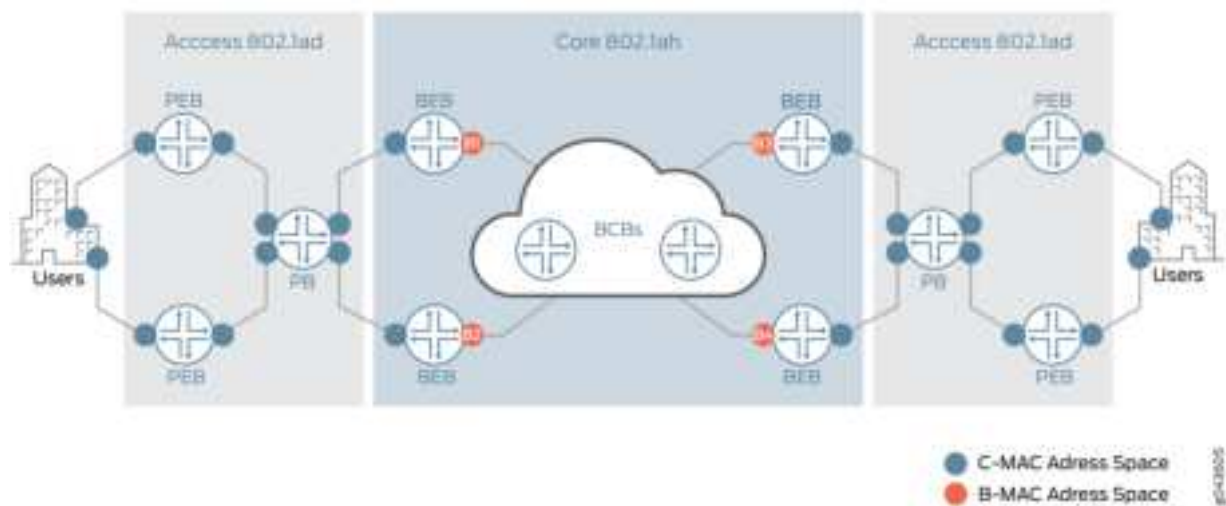
Figure 180: PBB Network Elements
