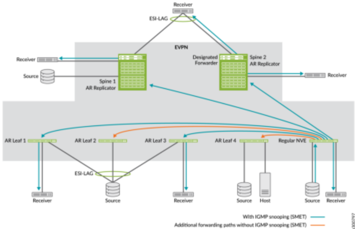
Figure 98: Multicast Source Traffic Ingress at a Regular NVE Device
