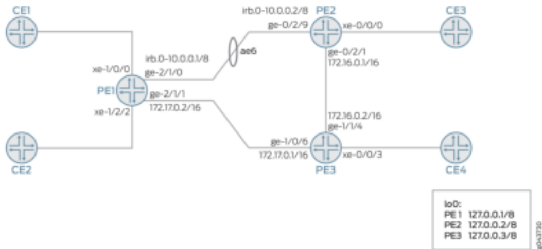
Figure 197: PBB with Single-Homed EVPN
