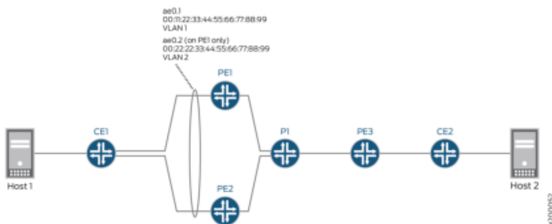
Figure 31: EVPN-MPLS Topology with Multihoming Active-Active
