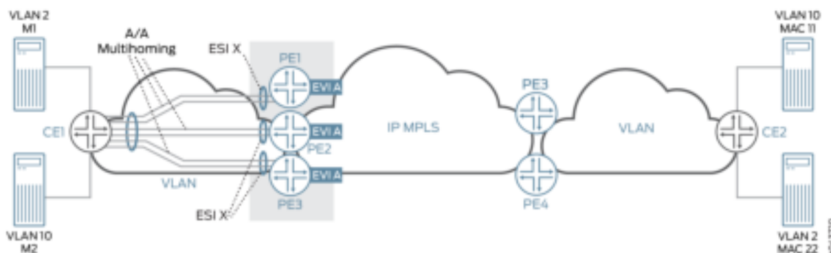
Figure 196: PBB-EVPN Redundancy Use Case
