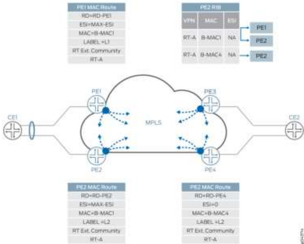
Figure 188: Ethernet MAC Routes Discovery
