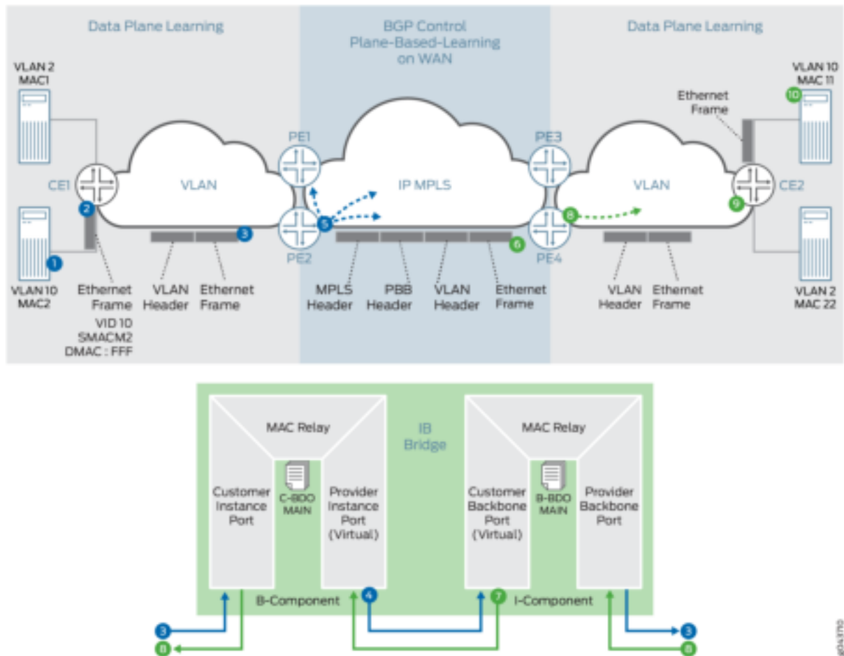
Figure 189: PBB-EVPN BUM Traffic Handling
