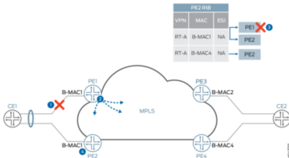
Figure 192: PBB-EVPN Segment Failure
