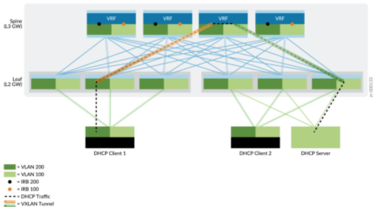
Figure 40: DHCP Relay Agent on Centrally-Routed Bridging Overlay
