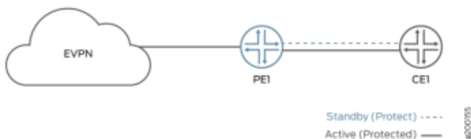
Figure 23: EVPN Active-Standby Multihoming on a Single PE Device
