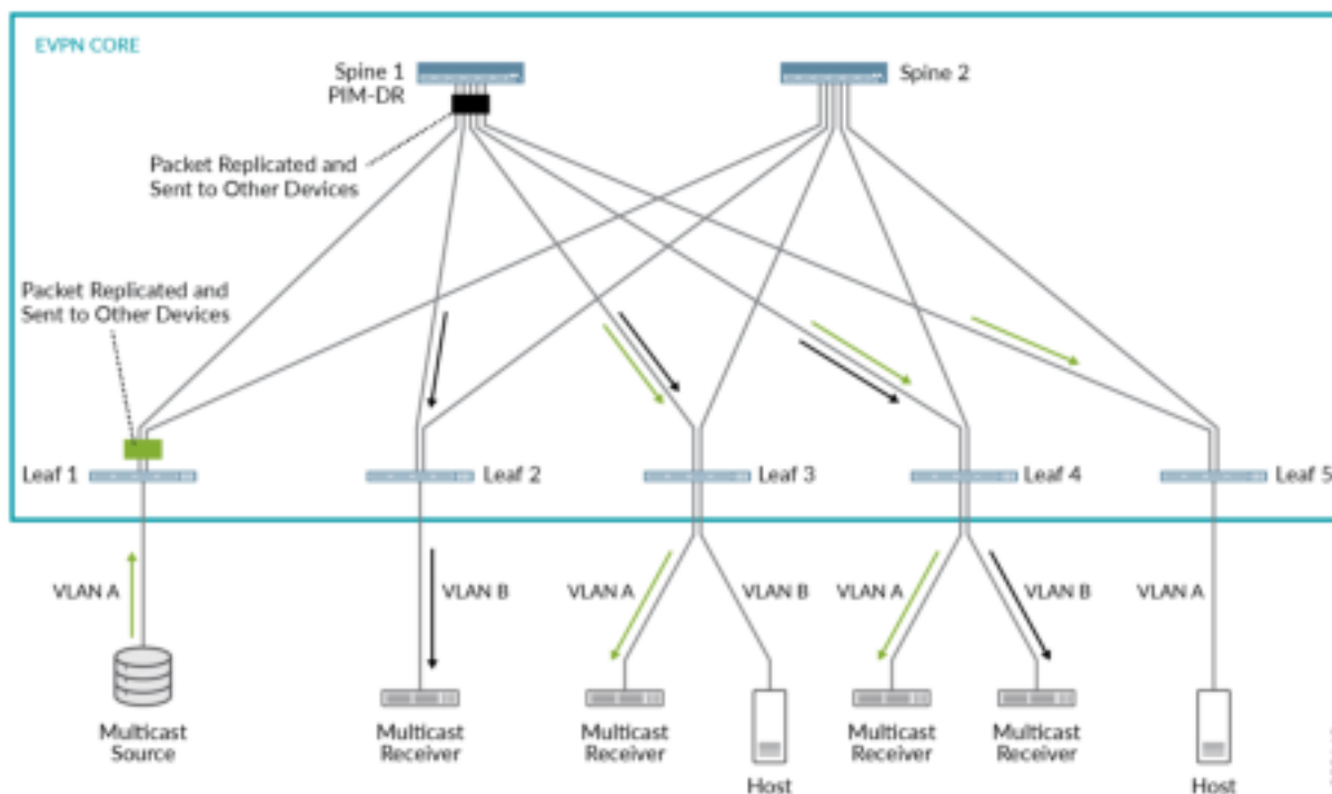
Figure 93: Inclusive Multicast Forwarding in a Centrally-Routed EVPN-VXLAN Network
