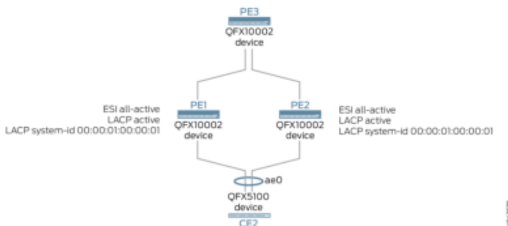
Figure 29: LACP Support in EVPN Active-Active Multihoming
