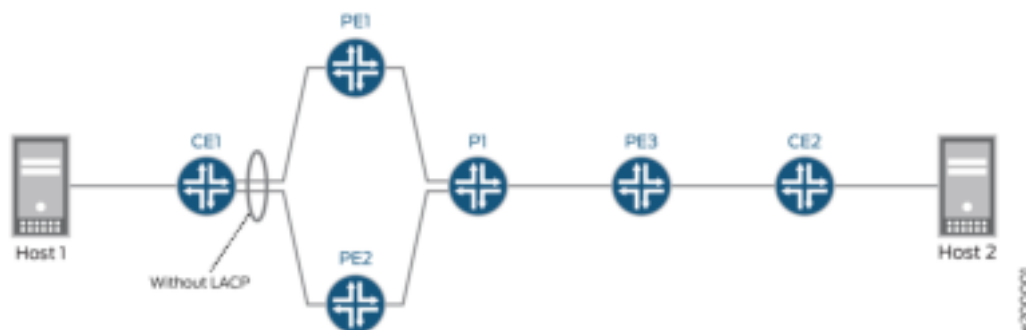
Figure 26: Simple EVPN Multihomed Topology
