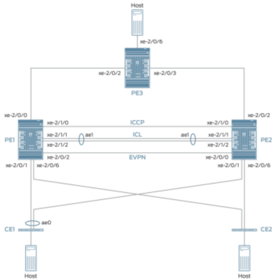
Figure 179: EVPN-MPLS Interworking With an MC-LAG Topology
