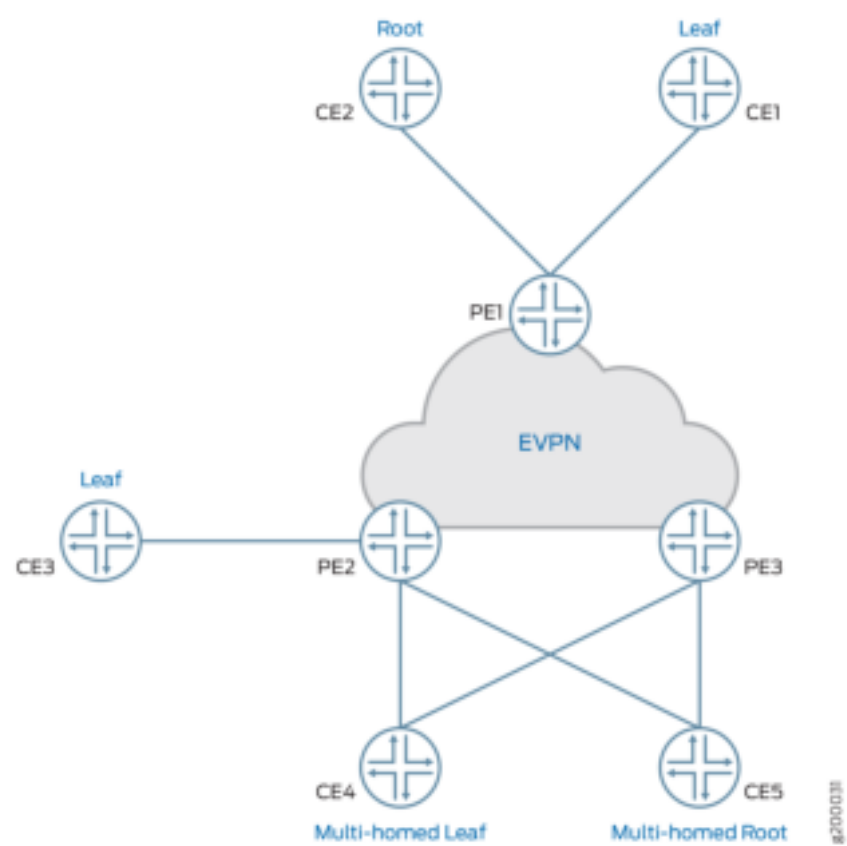
Figure 156: EVPN E-TREE Service
