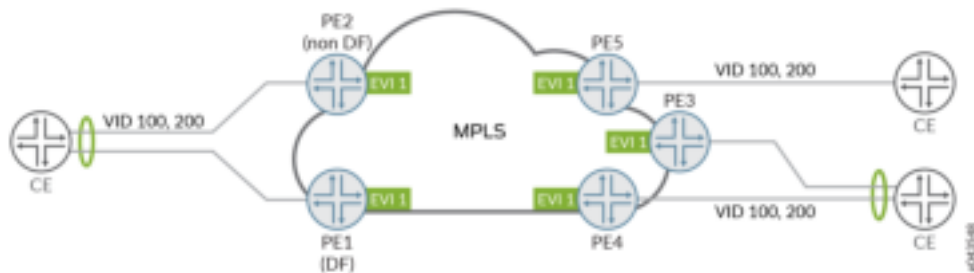
Figure 133: VLAN Bundle Network Topology
