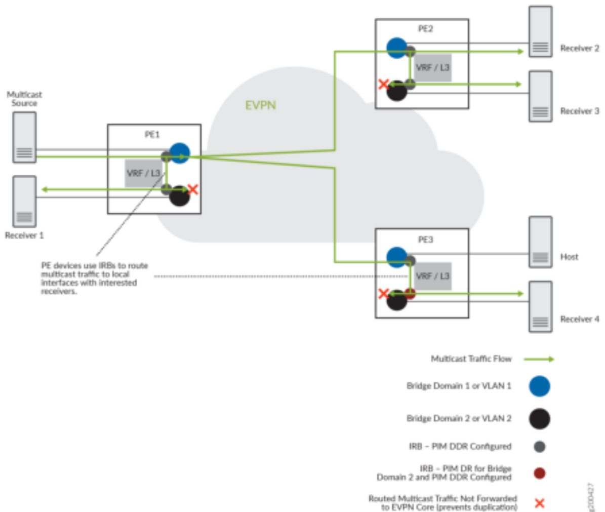
Figure 143: Routing Multicast Traffic Between Bridge Domains (or VLANs) with IRBs and PIM DDR in EVPN-MPLS
