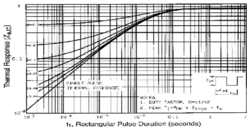
Fig. 11 - Maximum Effective Transient Thermal Impedance, Junction-to-Case
