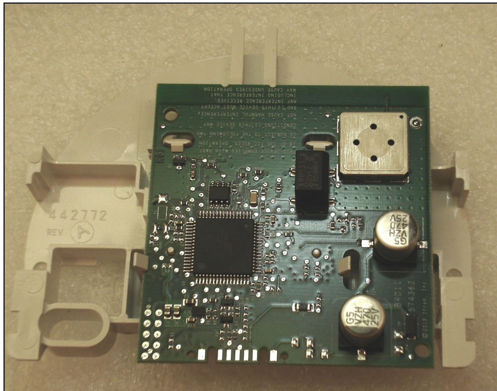
Figure 3: External Photo – Component Side
