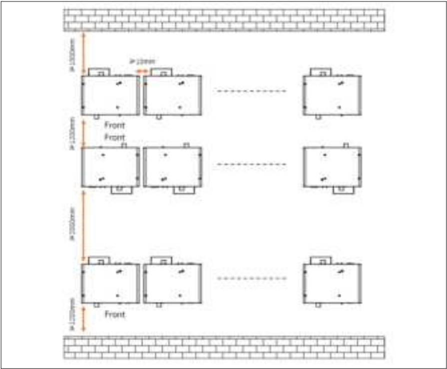
Fig2a. Clearance requirement
