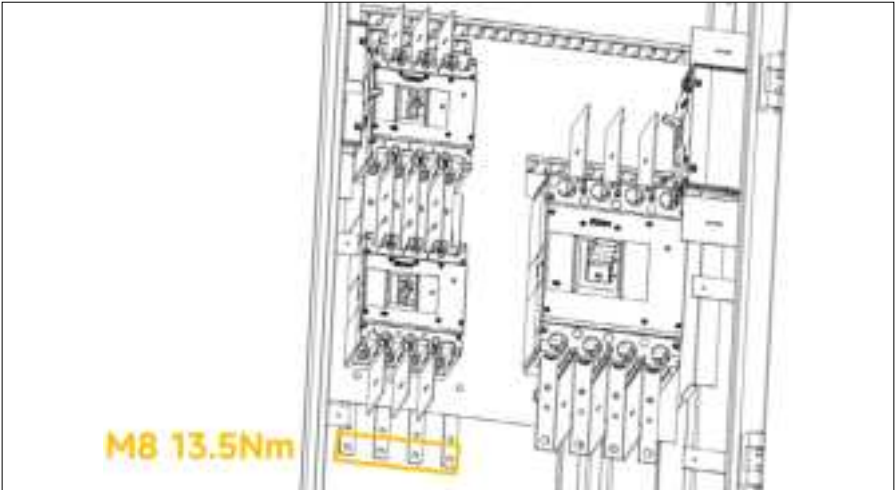
Figure 6. load side - copper busbar terminal connection
