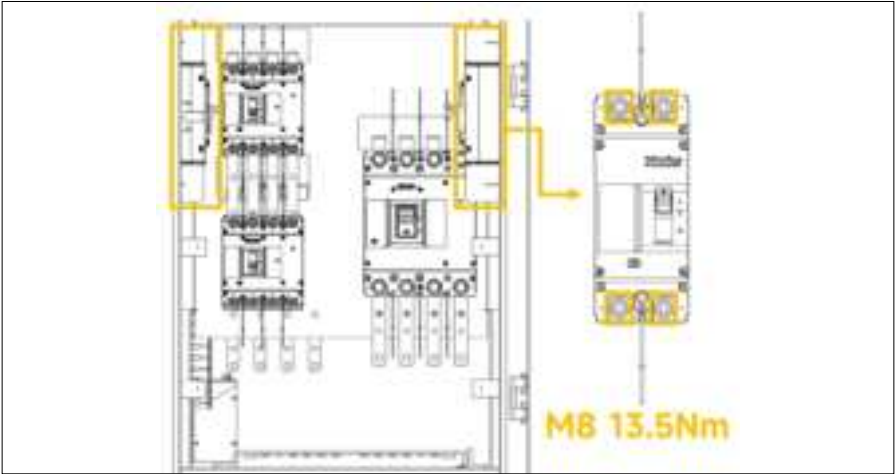
Figure 4. PV side - copper terminal connection
