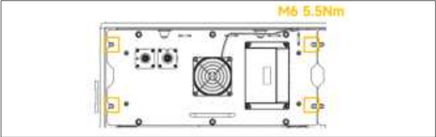
Figure 2. Screw position - pack
