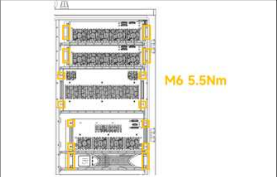
Figure 3. Screw position - module
