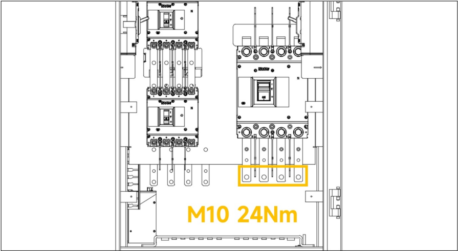
Figure 5. grid side - copper busbar terminal connection
