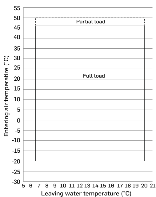
Operating map - cooling mode Standard unit 61AQ
