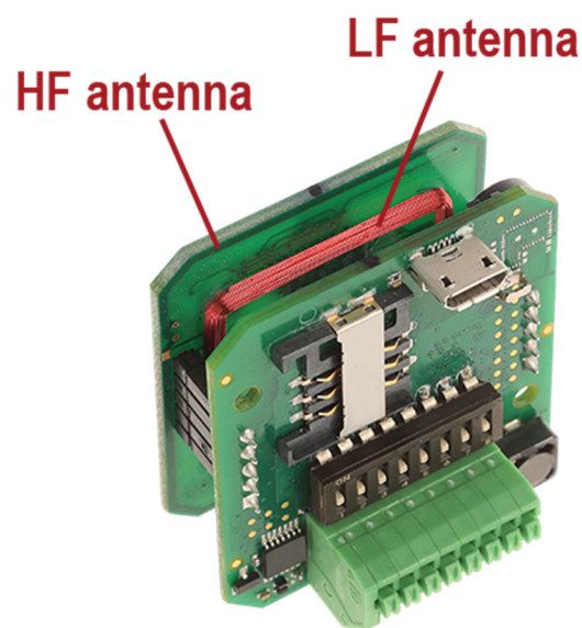
PCB contained in TWN4 Palon Compact Wall Light
