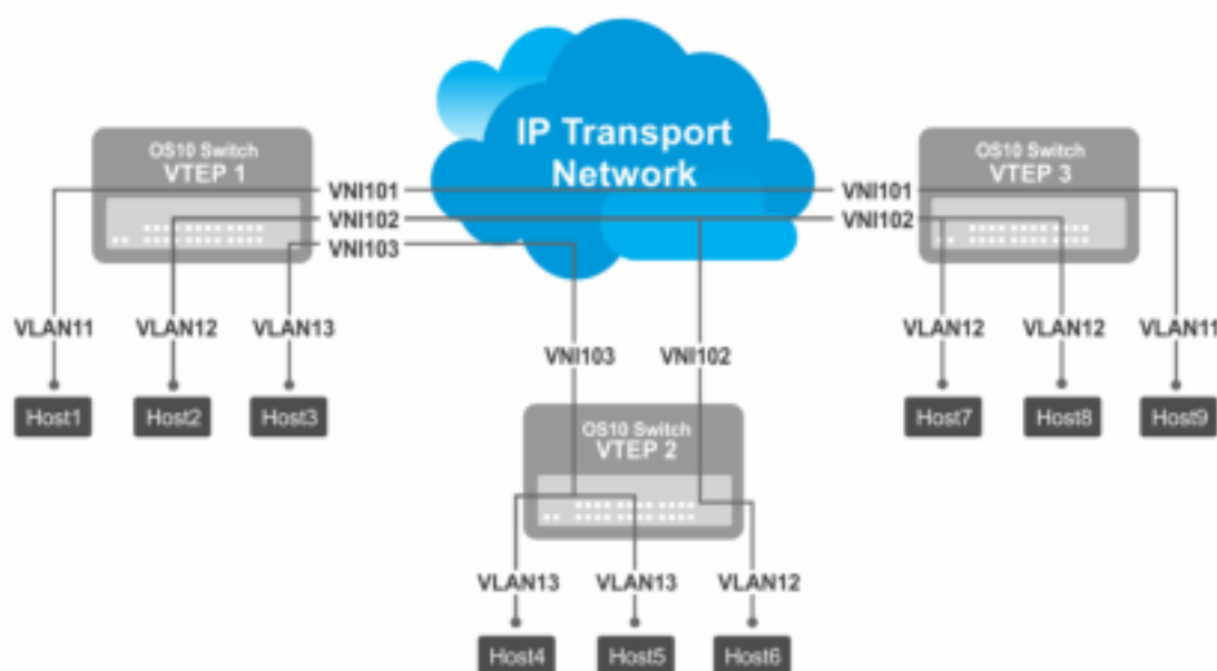
Figure 7. VXLAN topology
