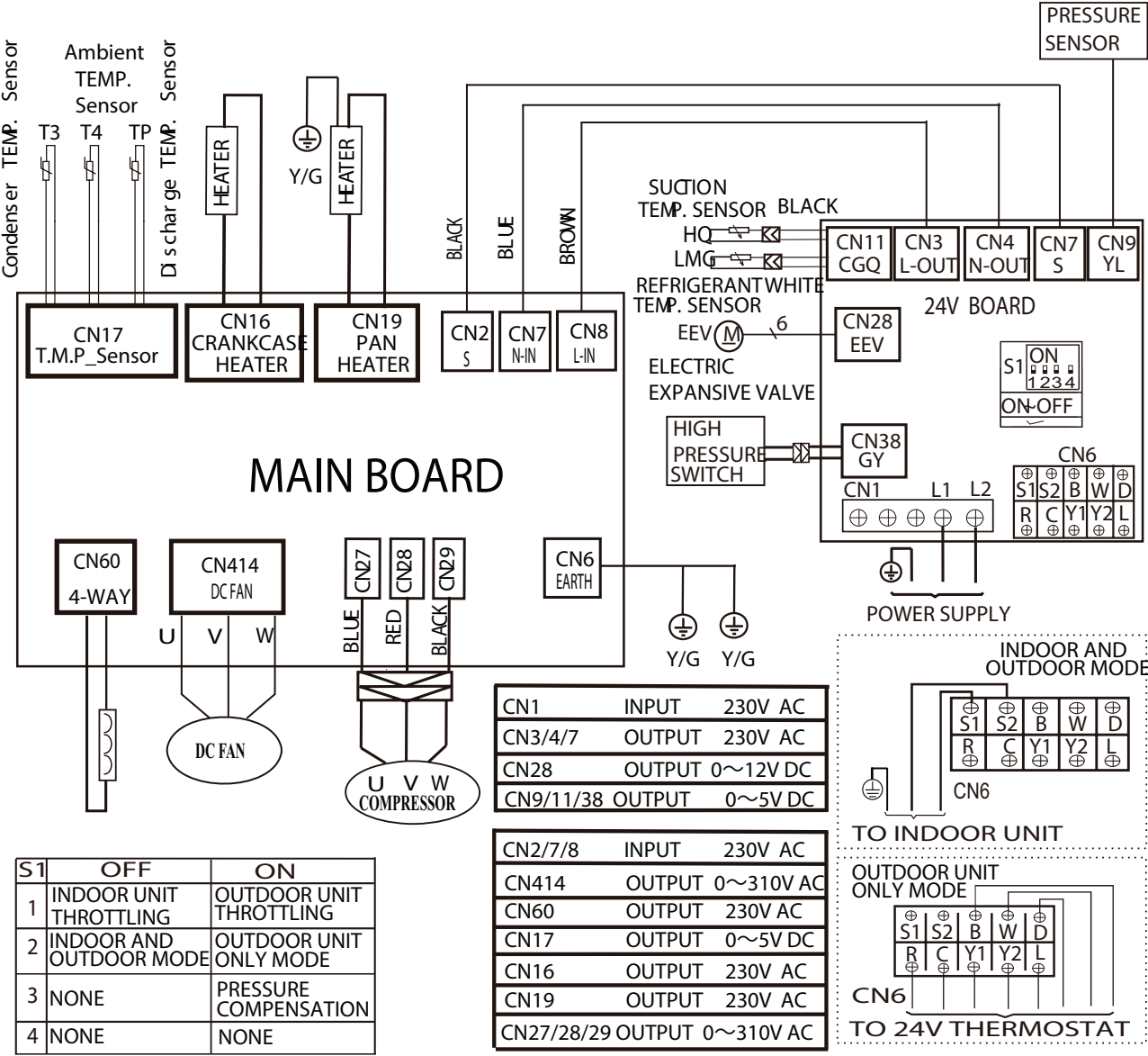
Fig. 15 — Wiring Diagram - Size 24K
