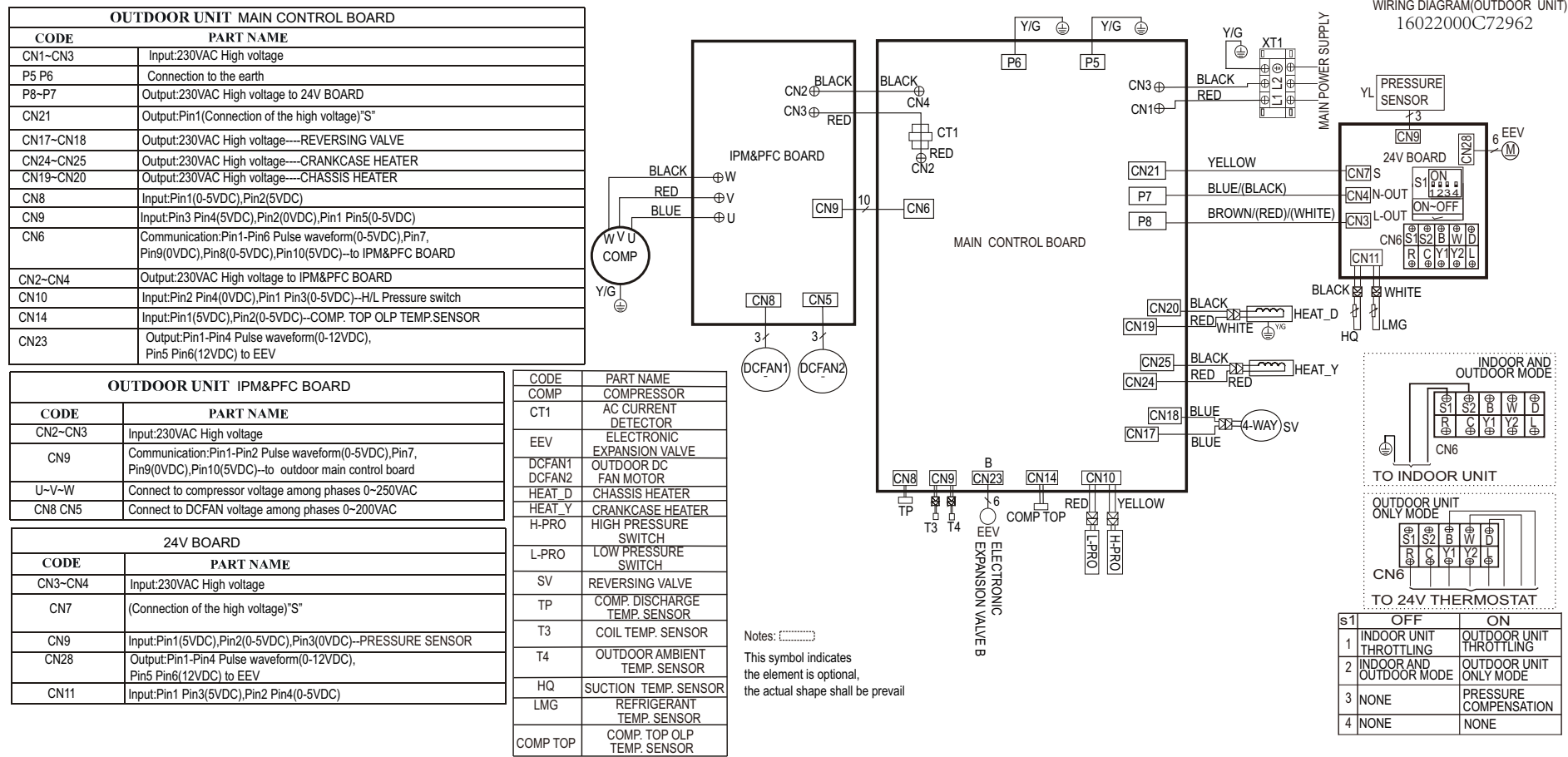
Fig. 14 —Wiring Diagram Sizes 36K-48K HH
