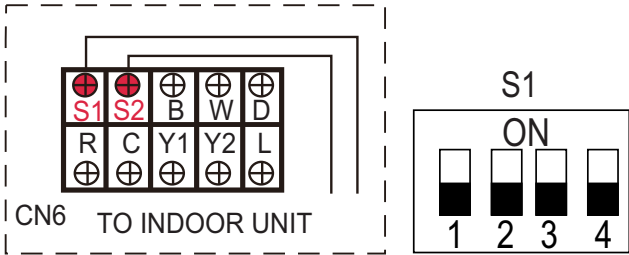
Fig. 3 —Option 1: Non-polarity RS485 Communication
