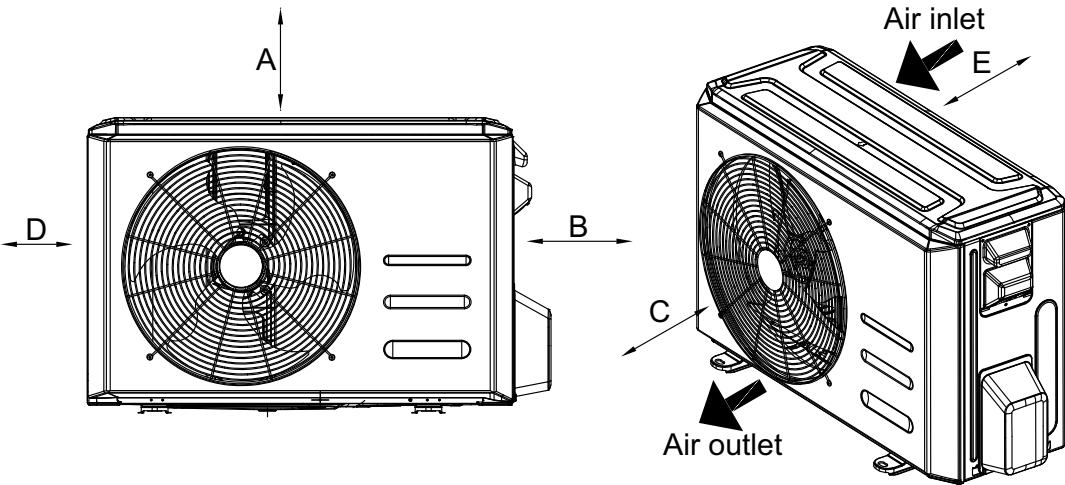
Fig. 5 —Clearances
