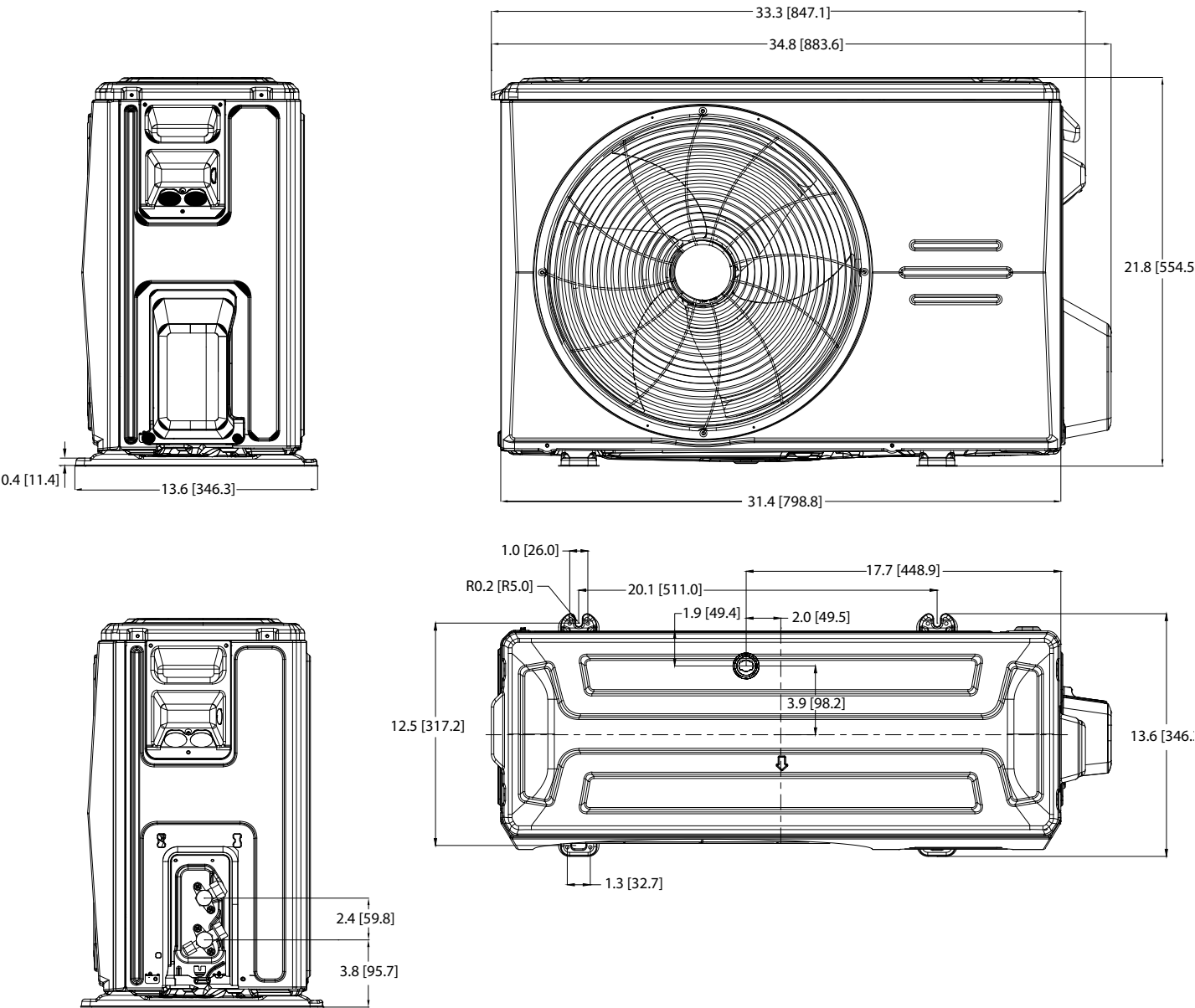
Fig. 2 —Dimension Size 18K
