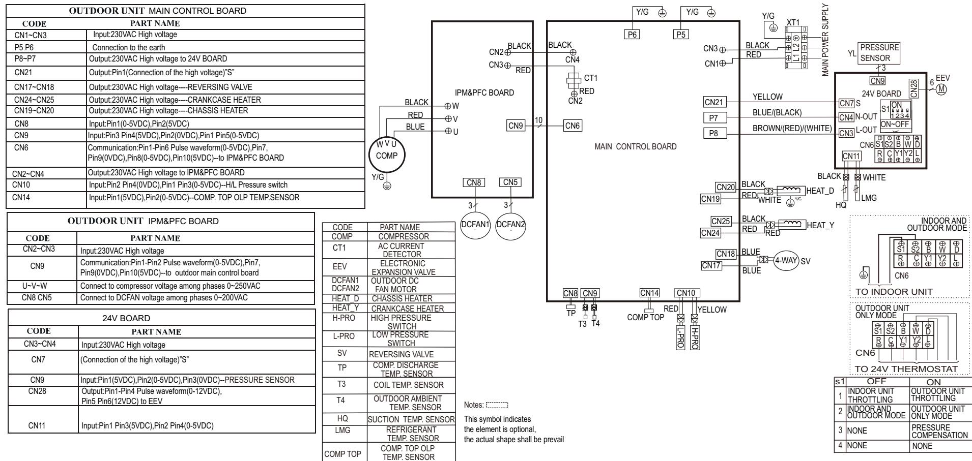
Fig. 17 —Wiring Diagram Sizes 48K-60K
