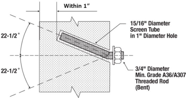
FIGURE 2—CONFIGURATION B (22½-DEGREE COMBINATION ANCHOR) 1
