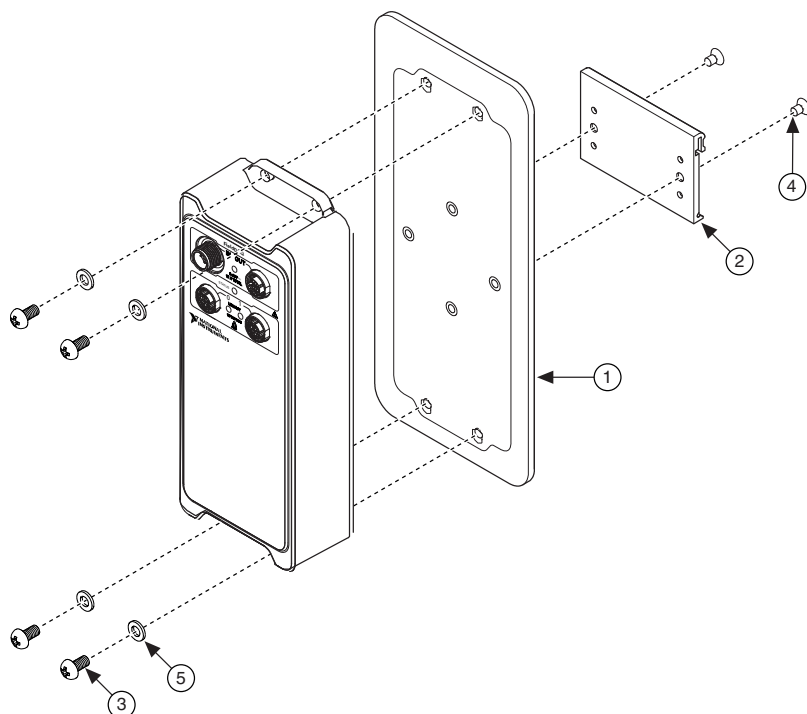
Figure 36. Attaching a FieldDAQ Device to the Bracket and DIN Rail Clip
