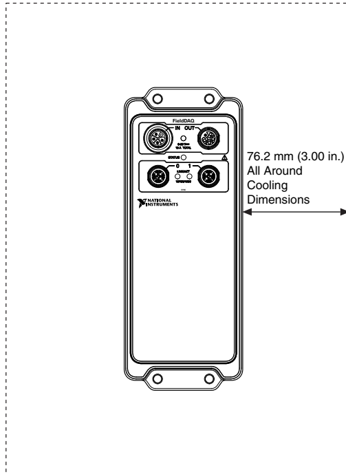
Figure 30. Cooling Dimensions
