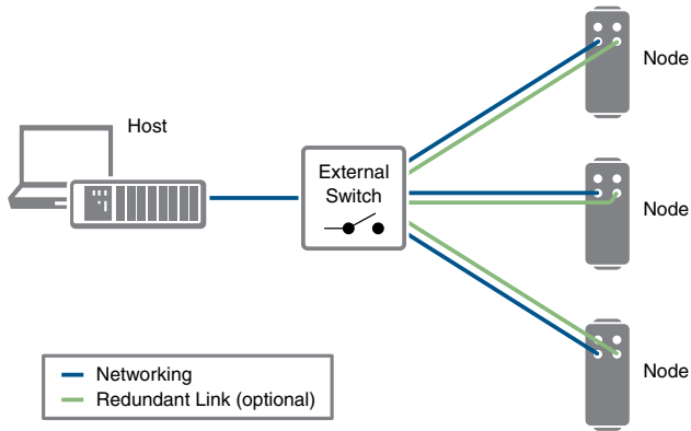
Figure 24. Star Topology
