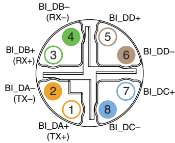
Figure 21. Ethernet Connector Pinout
