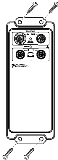
Figure 35. Fastening the Device to the Surface
