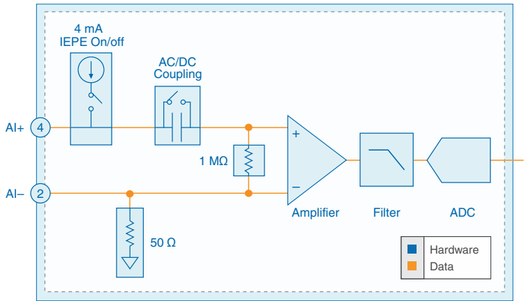
Figure 8. FD-11634 Input Circuitry
