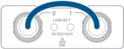
Figure 28. Connecting Port 0 and Port 1
