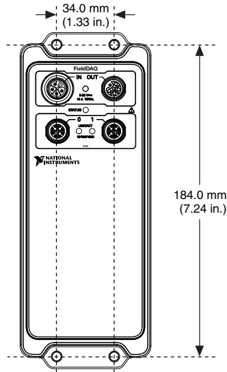
Figure 34. Surface Mounting Dimensions
