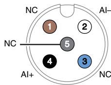
Figure 10. FD-11634 Pinout
