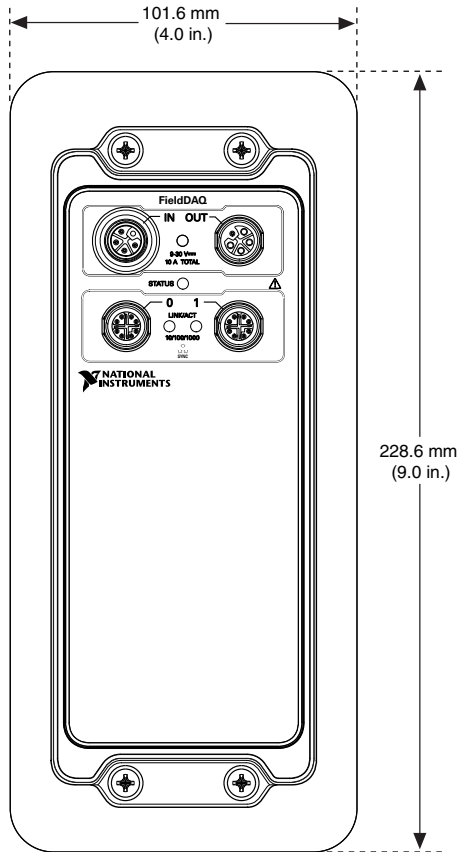
Figure 38. FD-11960 Dimensions
