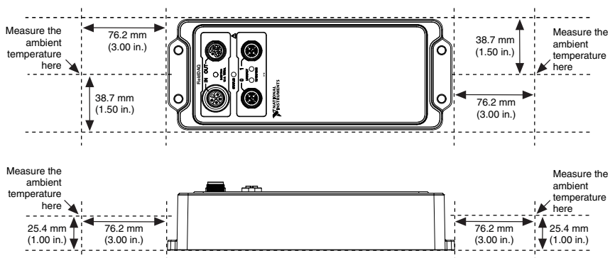
Figure 32. Ambient Temperature Locations, Horizontal Mounting Configuration
