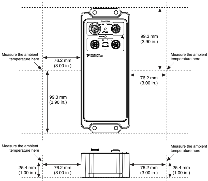
Figure 33. Ambient Temperature Locations, Vertical Mounting Configuration
